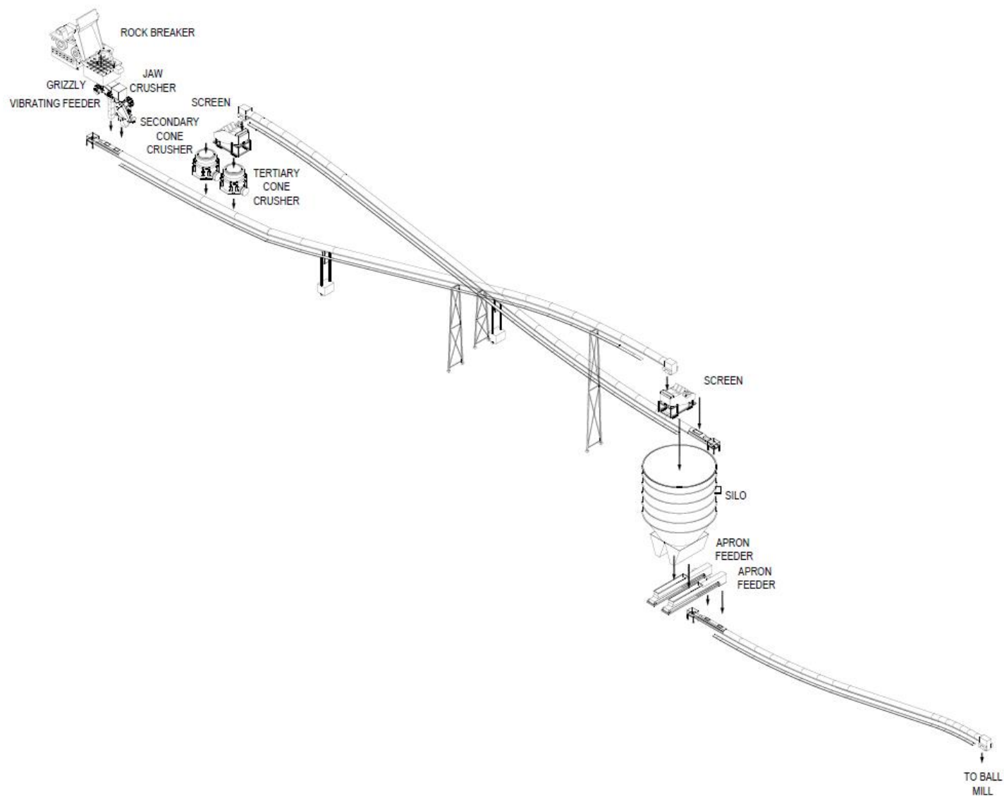
Figure 17-1: Process Flow Diagram (Crushing section)
