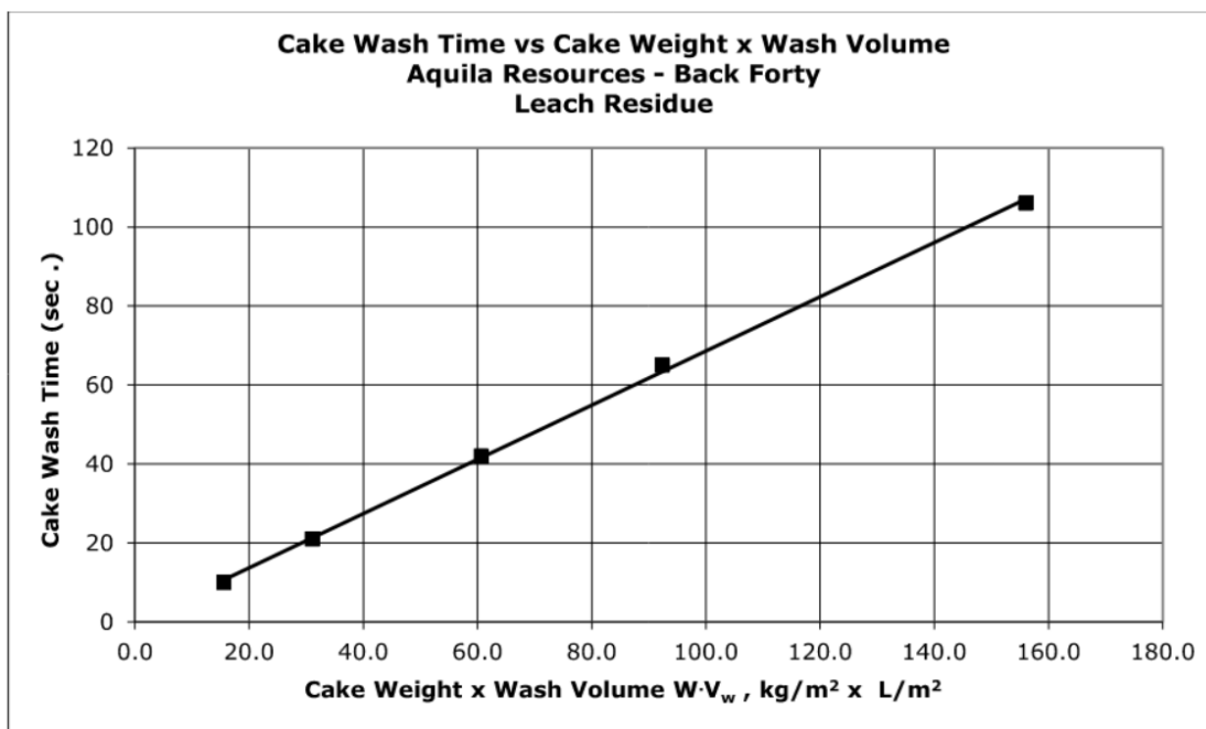
Figure 13-17: Cake Wash Time Versus Cake Weight x Wash Volume – Aquila Resources – Back Forty Leach Residue
