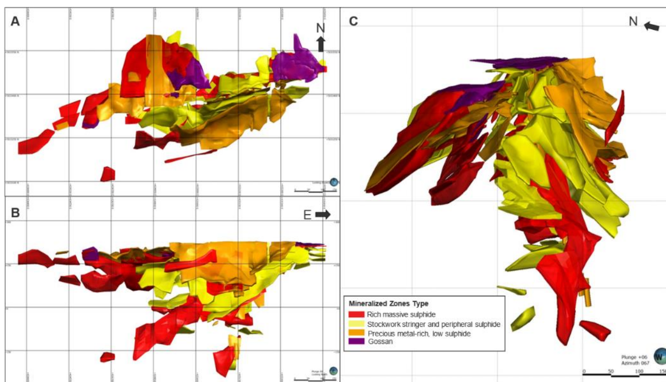
Figure 7-10: 3D Model of the Mineralized Zones of the Back Forty Deposit
