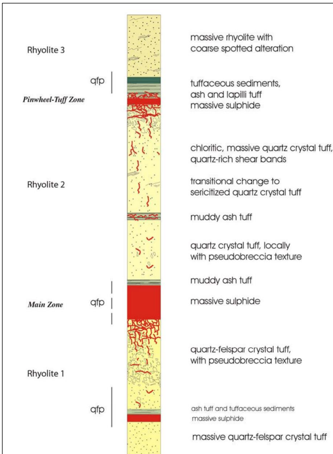
Figure 7-11: Back Forty Massive Sulfide Stratigraphic Column
