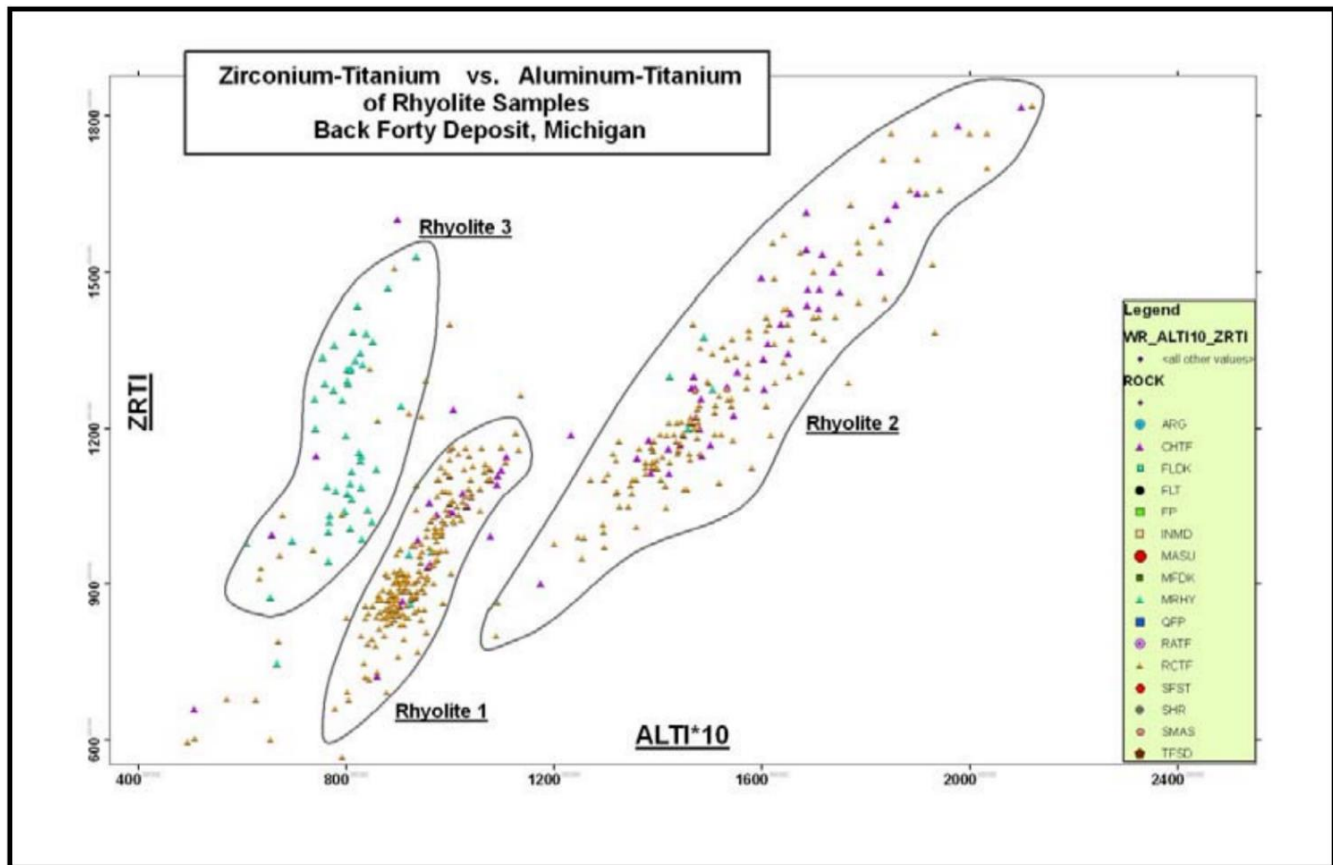
Figure 7-12: Zr-Ti Versus Al-Ti Ratios of Rhyolites at the Back Forty Project
