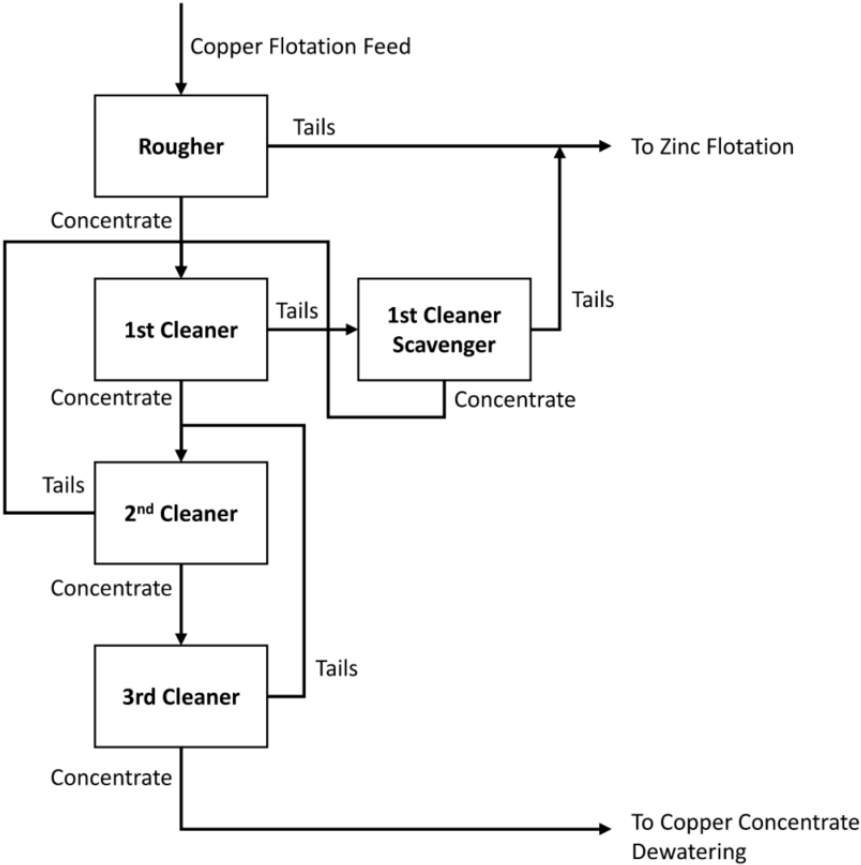
Figure 17-3: Copper Flotation Circuit
