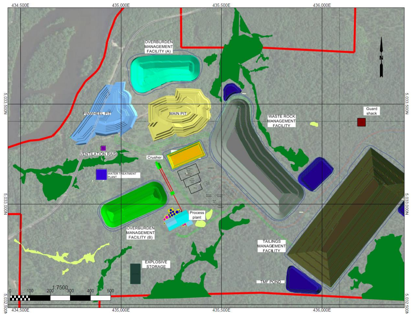
Figure 16-4: Ultimate Pit, Overburden Stockpile and Waste Rock Dump
