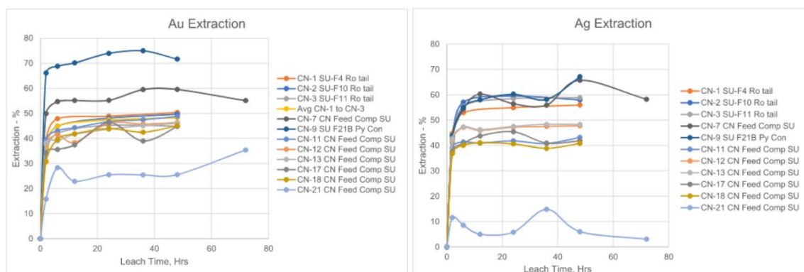
Figure 13-11: Comp SU Direct Cyanidation Extraction
