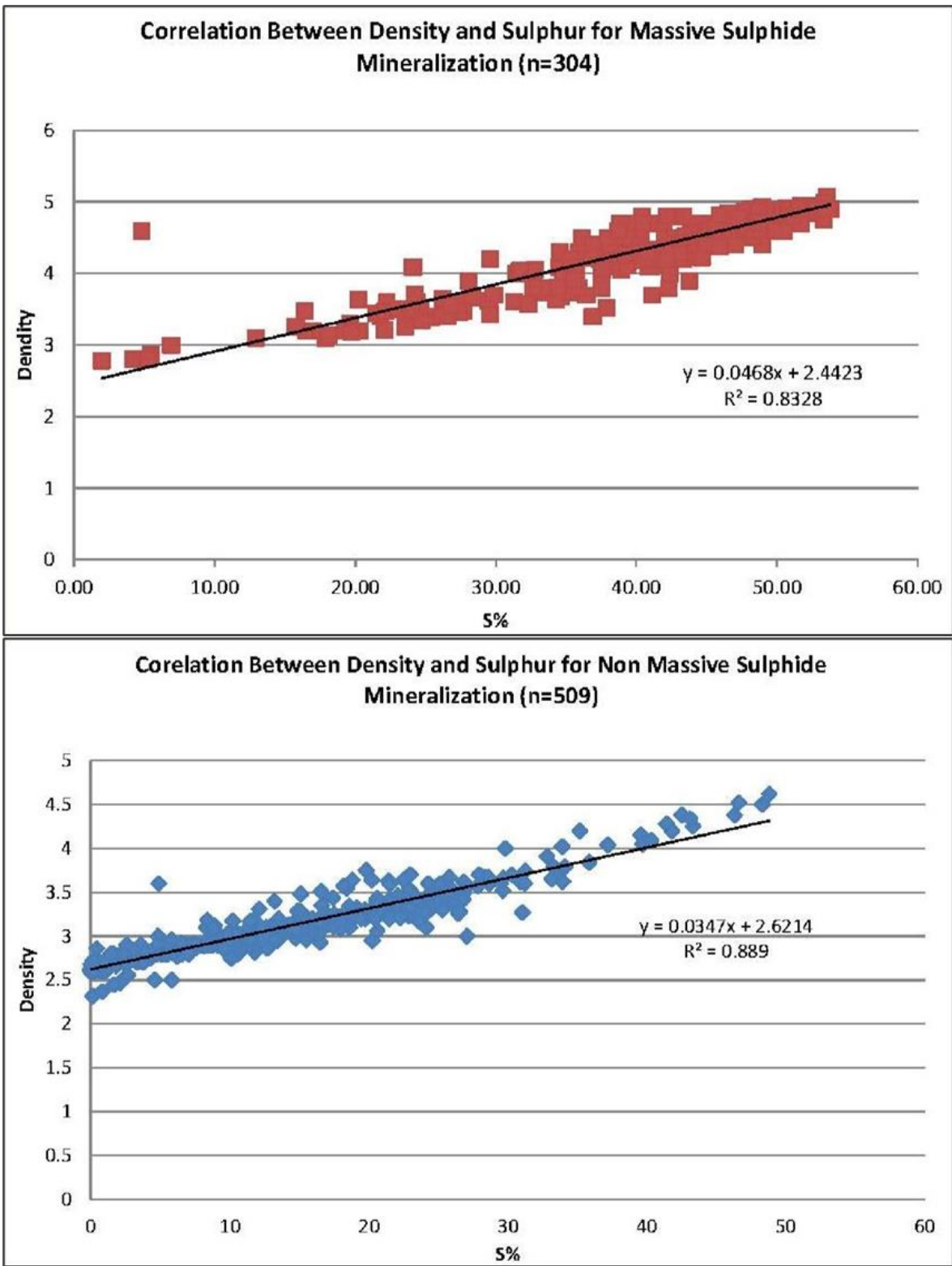
From Bradfield et al., 2020 Figure 14-5: Correlation Between Bulk Density and Sulfur
