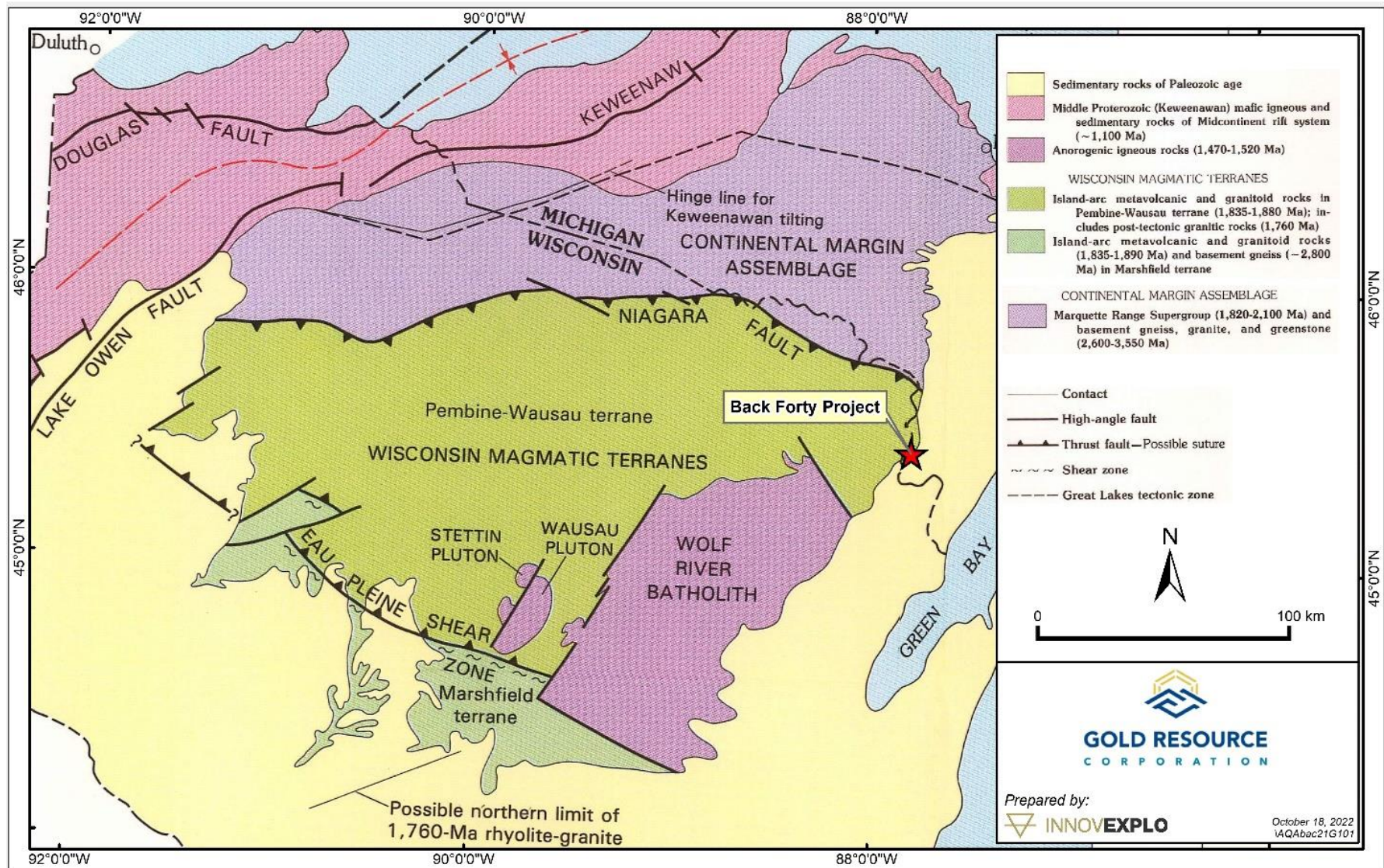
Figure 7-2: Geological Map of Northern Wisconsin and Western Michigan
