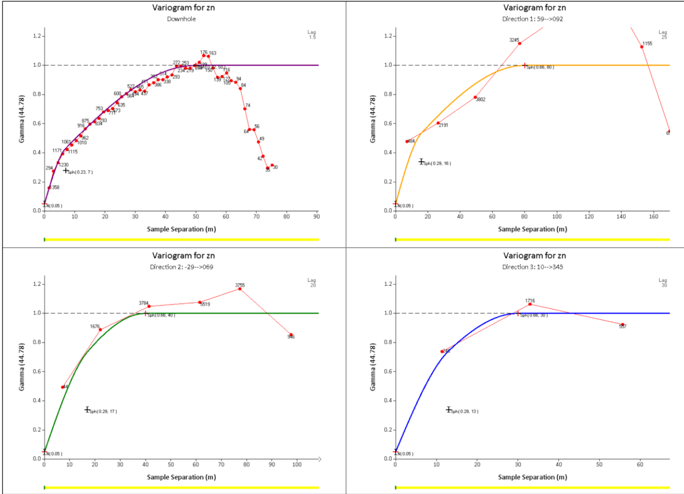
Figure 14-6: Variography Study for Zinc in the Main MS1 Zone
