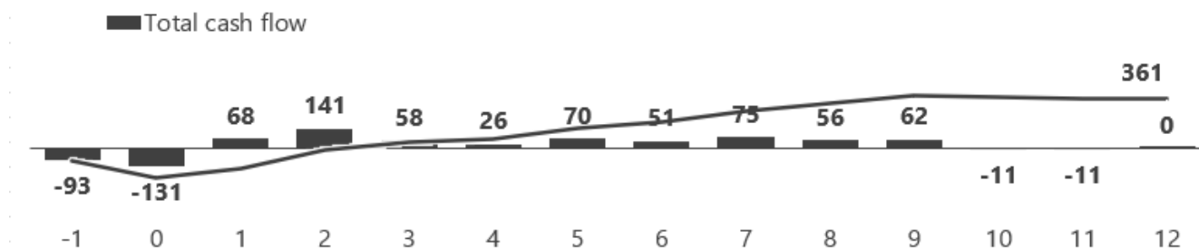
Figure 22-3: Cash Flow Profile
