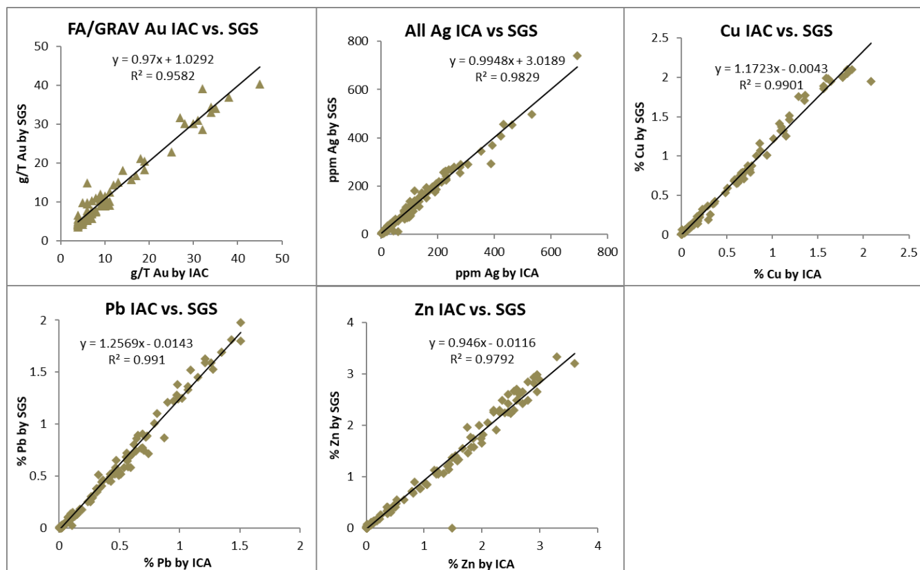
Figure 11-2: Linear Regression Graphs Comparing IAC versus SGS Assay Results
