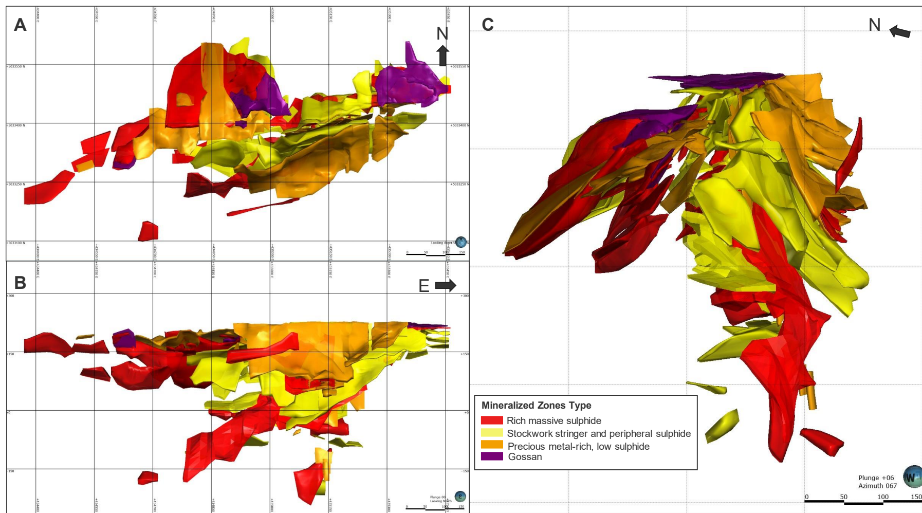
Figure 14-2: Mineralized Solids of the Back Forty Project
