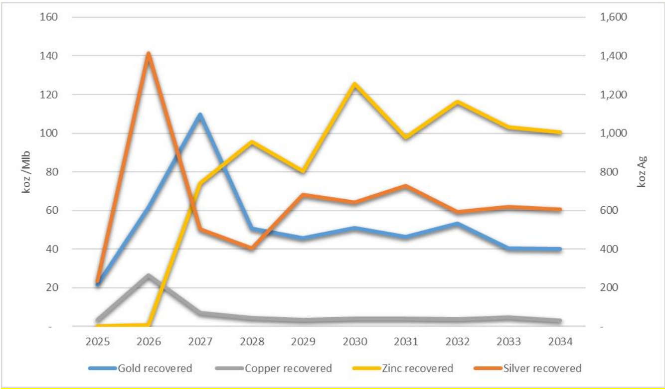
Figure 22-2: Recovered Metal Profile
