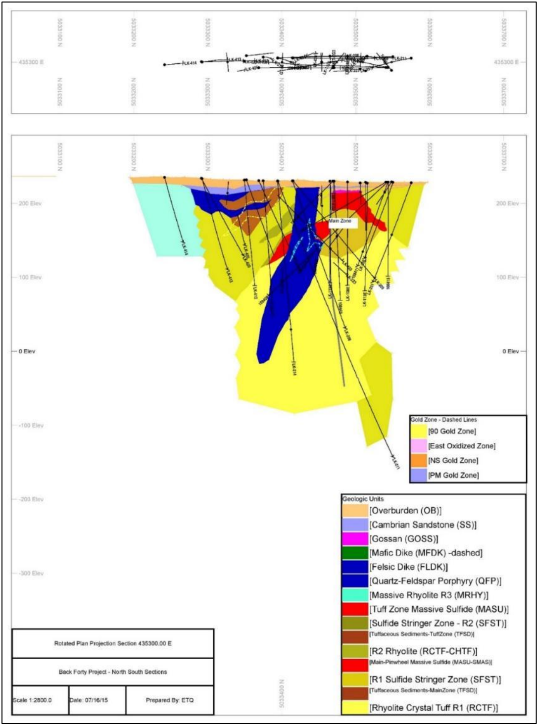
Figure 7-7: Typical Cross-Section through the Eastern Portion of The Back Forty Deposit
