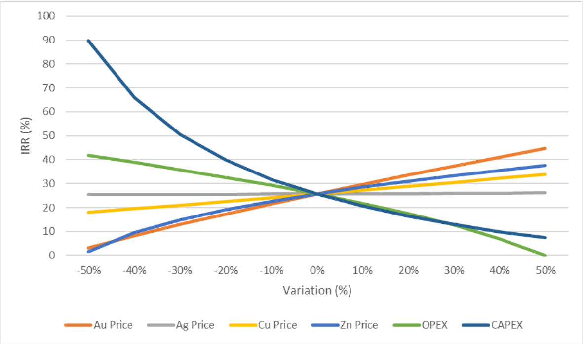
Figure 22-8: Spider Chart for Variation of Metal and Expenses on IRR
