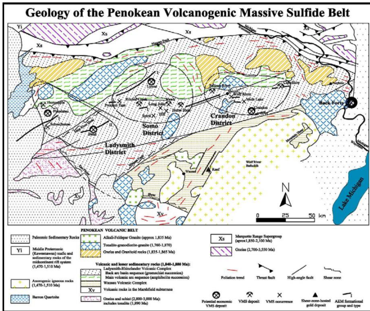
Figure 7-3: Geological Map of The Penokean Volcanic Belt with Location and Distribution of the VMS Districts
