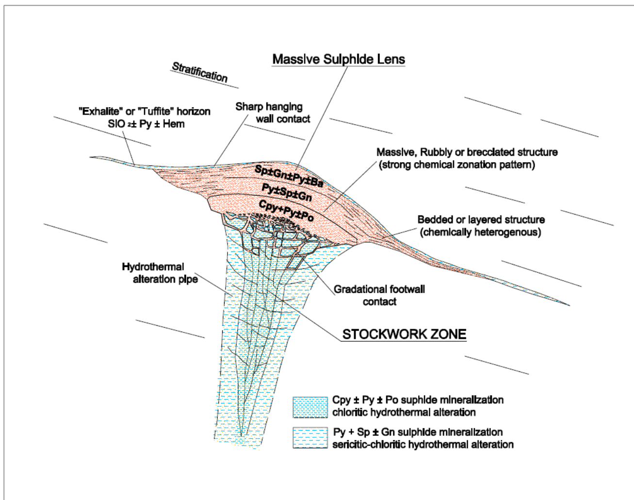
Figure 8-1: Principal Characteristics of an Idealized VMS Deposit
