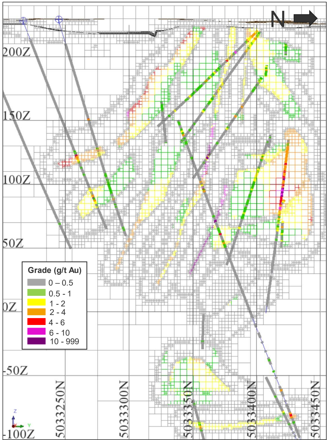
Figure 14-7: Gold Grade Distribution for Section 435140E
