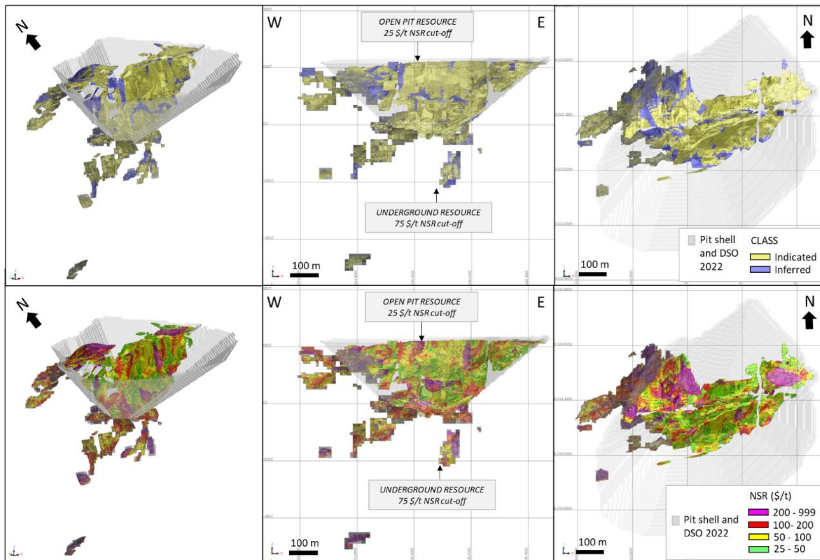
Figure 14-10: Isometric, Longitudinal and Plan Views Showing the Classified Mineral Resources and the Interpolated NSR Constrained in Optimized Pit-shells and DSO Stope Designs
