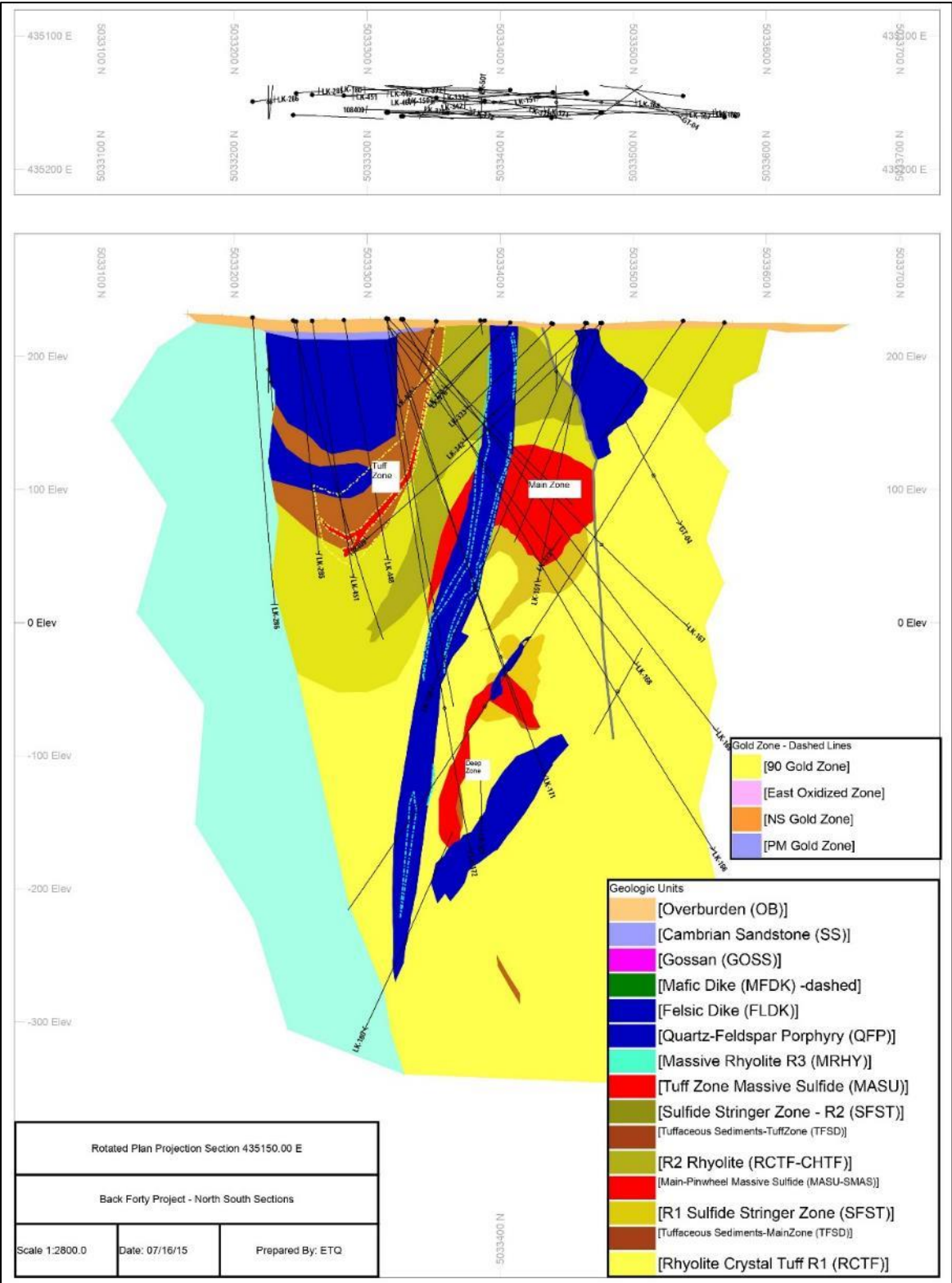
Figure 7-8: N-S Cross-Section through the Central Portion of the Back Forty Deposit
