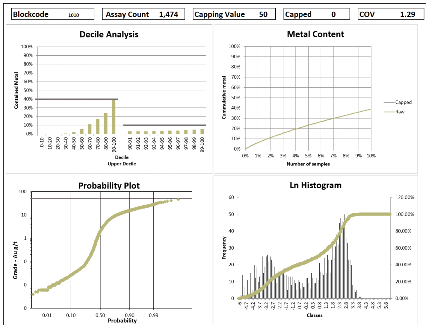
Figure 14-3: Example of Graphs Supporting the None Capping of Zinc for the 1010 Zone
