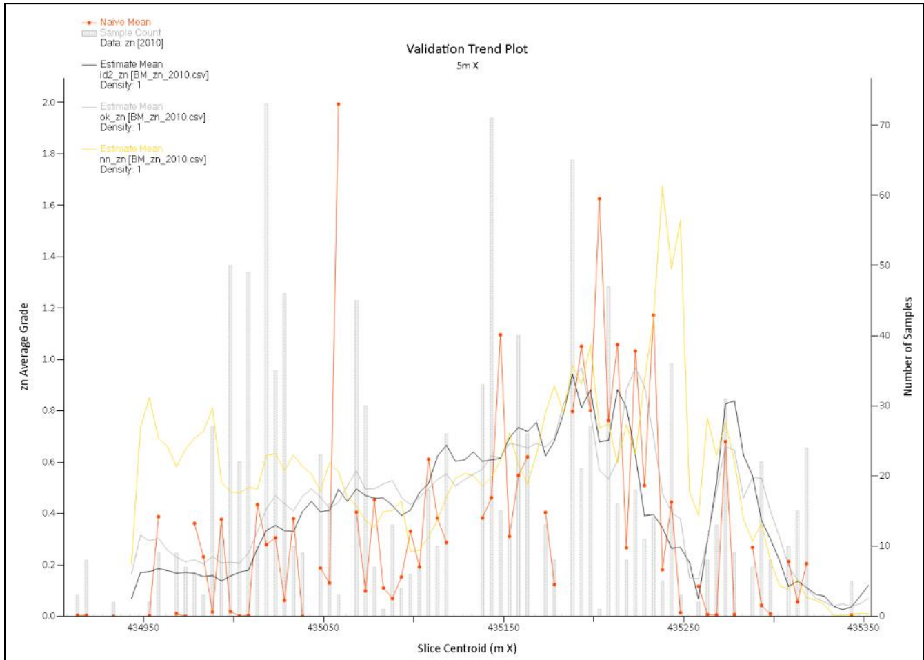
Figure 14-9: Validation Swath Plot of Zone 2010 for Zinc (East Direction)
