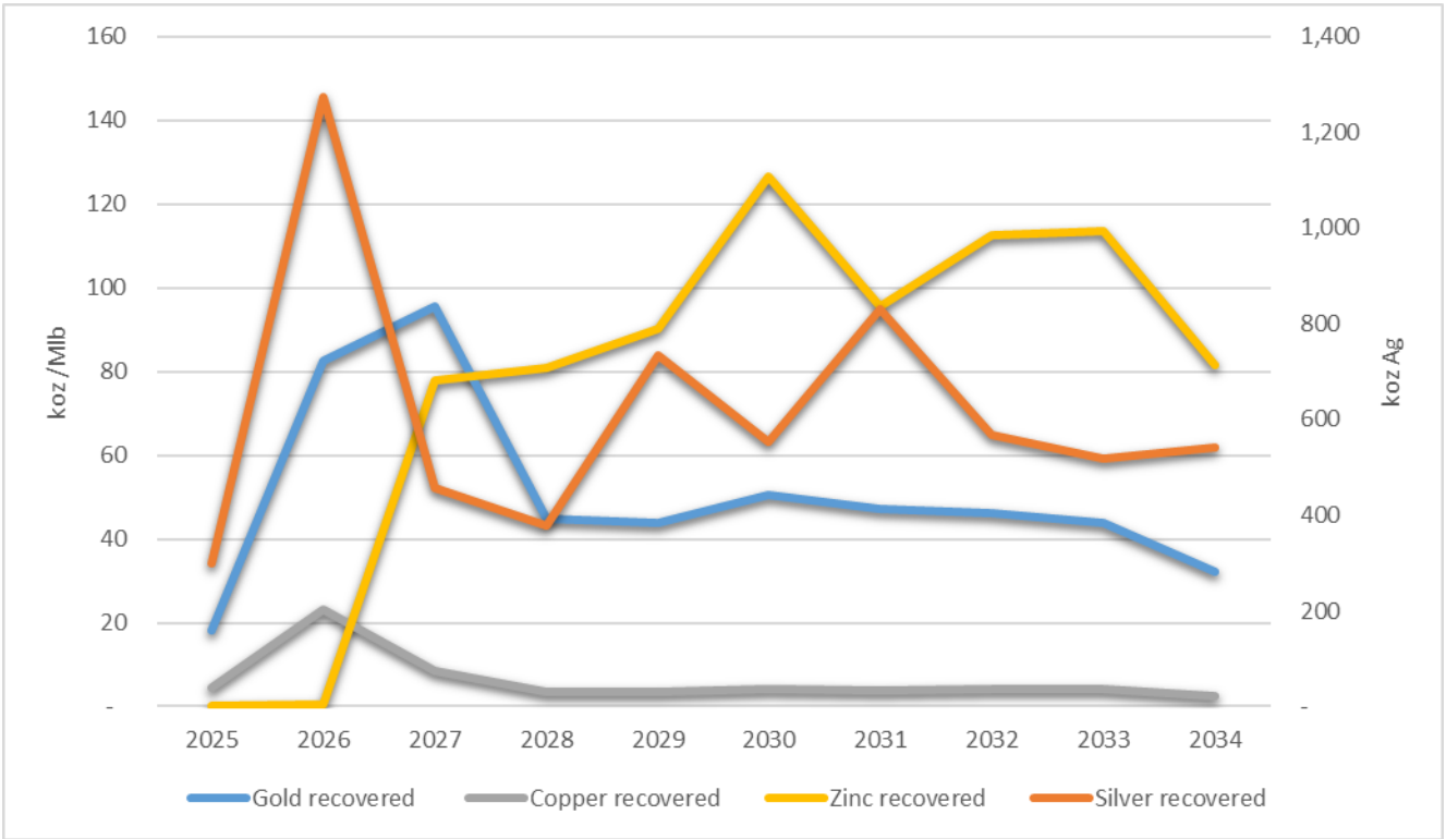
Figure 22-5: Recovered Metal Profile for Case Without Inferred Material
