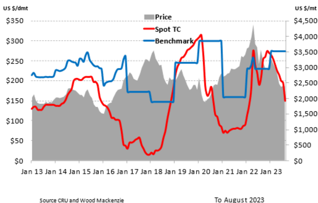
Figure 19-1: 10 Year Chart- Zinc Spot and Benchmark TCs versus LME Zinc Price
