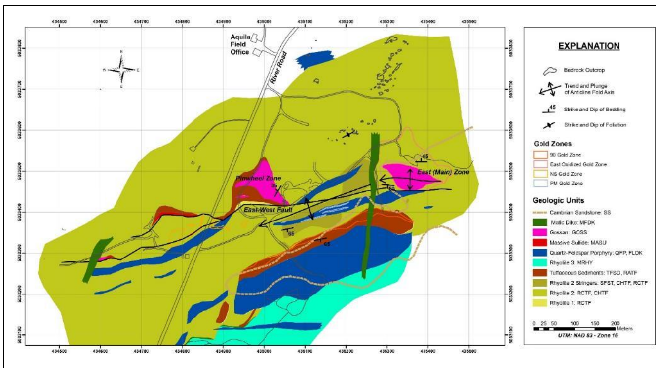
Figure 7-6: Geological Map of the Back Forty Deposit
