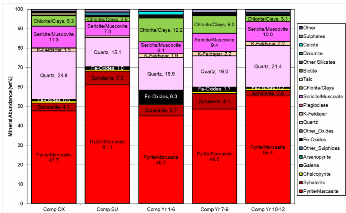
Figure 13-3: Modal Mineral Distribution
