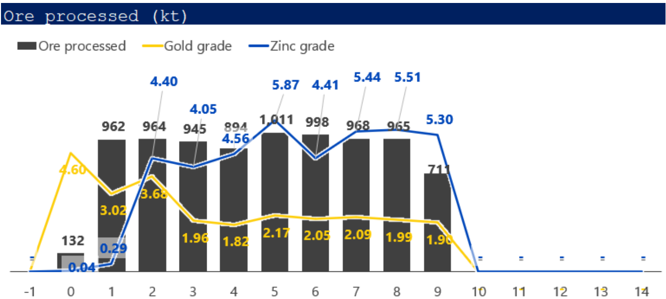
Figure 22-4: Materialized Material Processed and Grade Profiles for Gold and Zinc for Case Without Inferred Material
