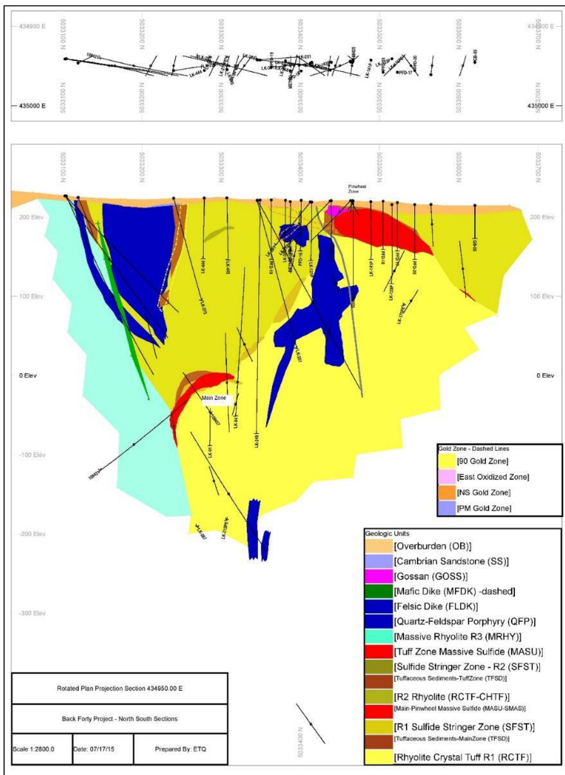
Figure 7-9: Typical Cross-Section through the Western Portion of the Back Forty Deposit
