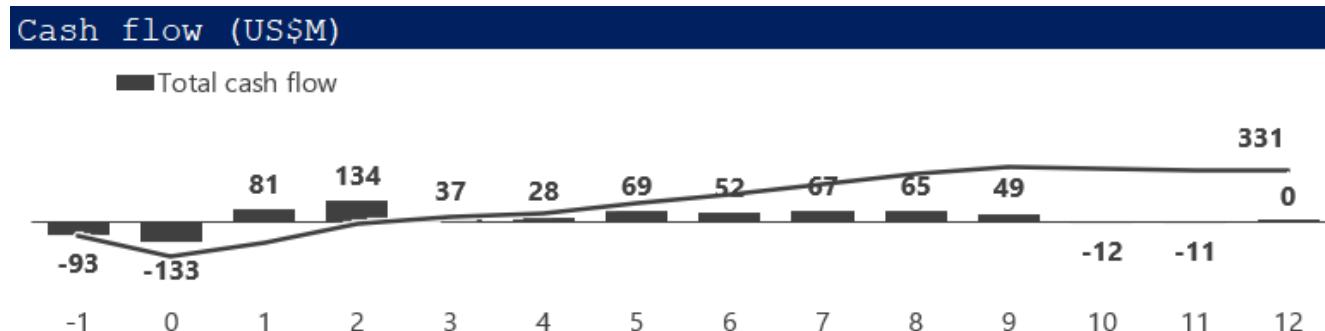
Figure 22-6: Cash Flow Profile for Case Without Inferred Material
