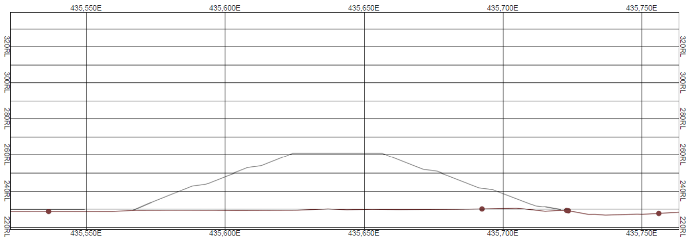
Figure 18-7: Typical Cross-Section of the WRMF
