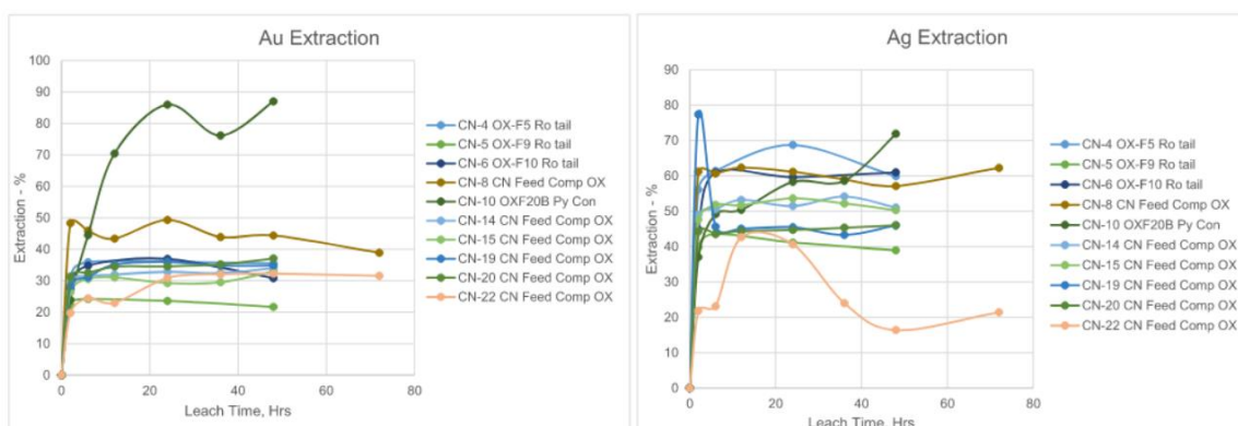
Figure 13-12: Comp OX Direct Cyanidation Extraction
