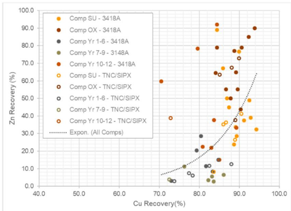
Figure 13-8: Copper Rougher Stage - Cu Versus Zn Selectivity
