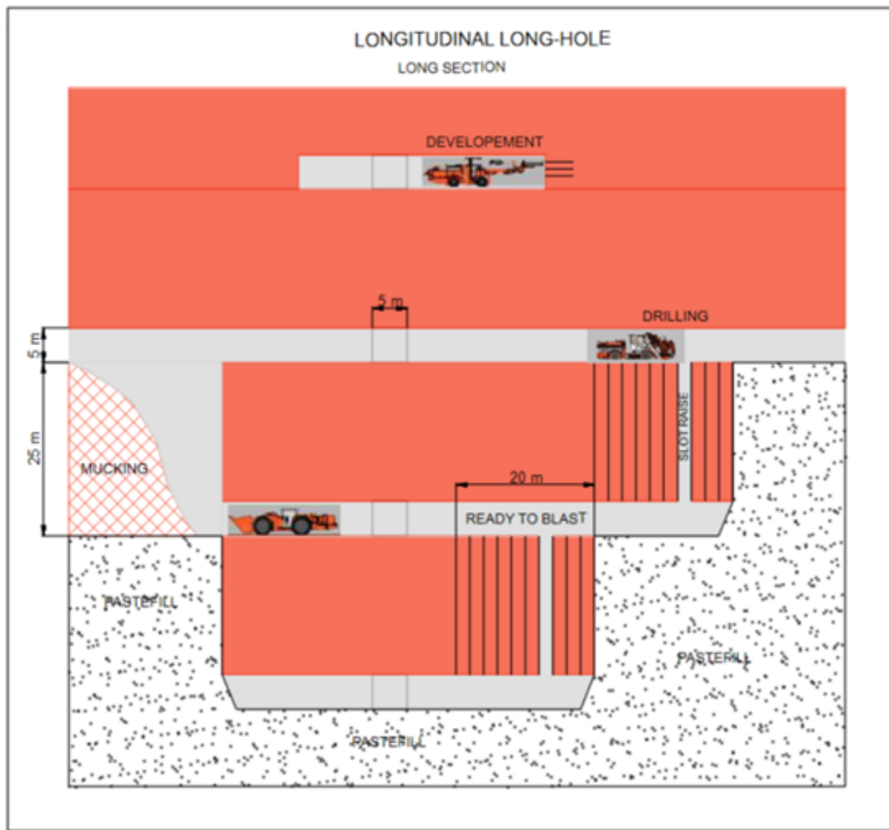
Figure 16-11: Sectional View of Longitudinal Longhole Stope
