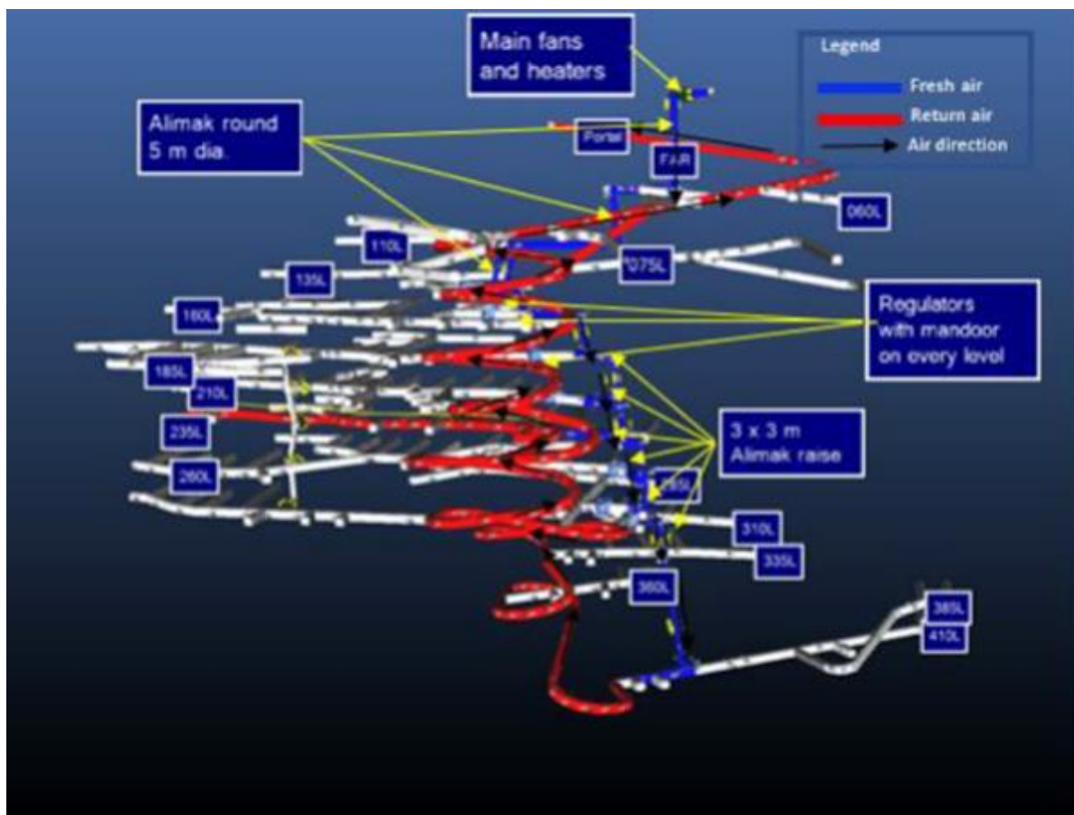
Figure 16-15: Ventilation Network Isometric View
