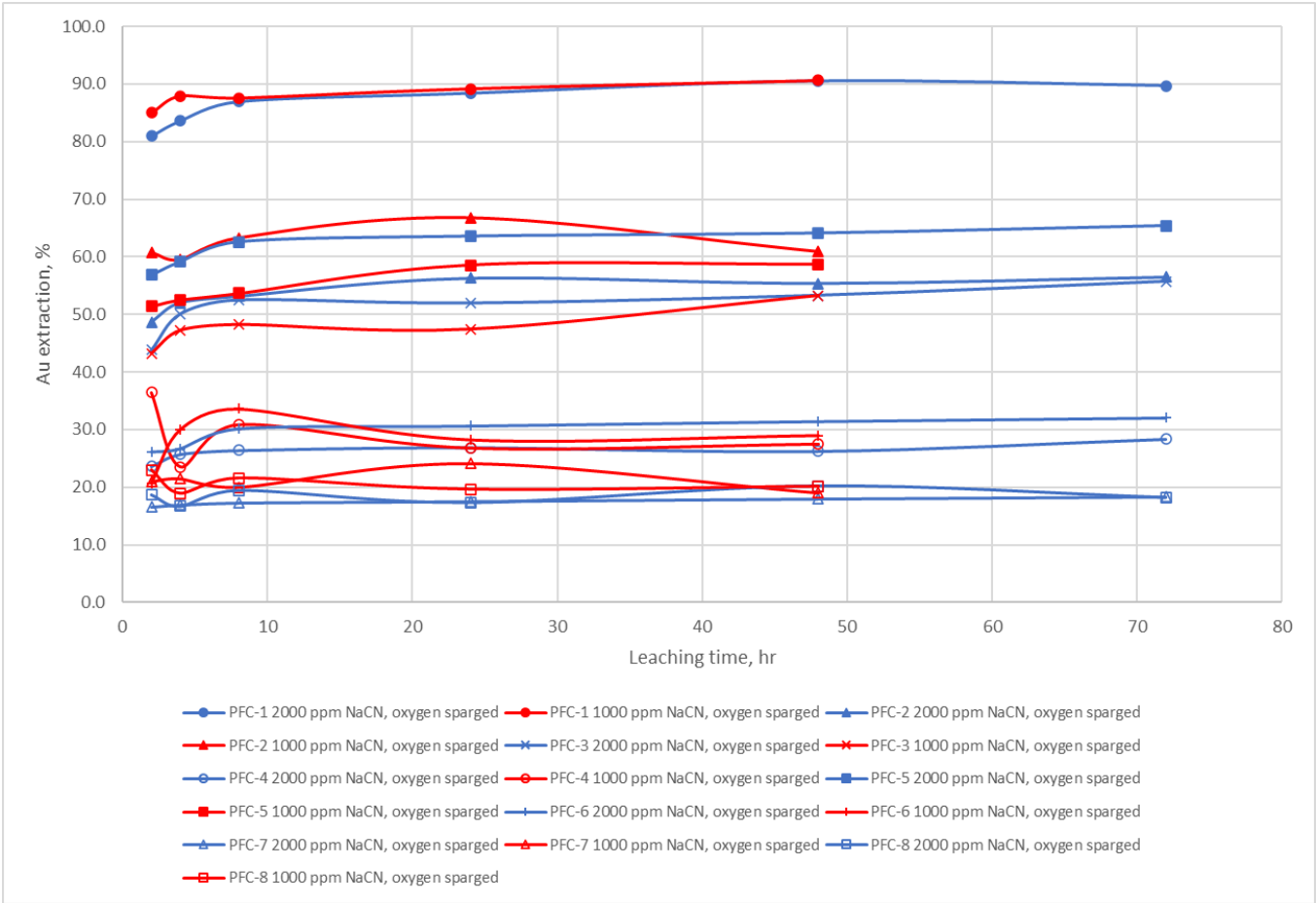
Figure 13-23: Leaching Performance Under Different Cyanide Concentrations
