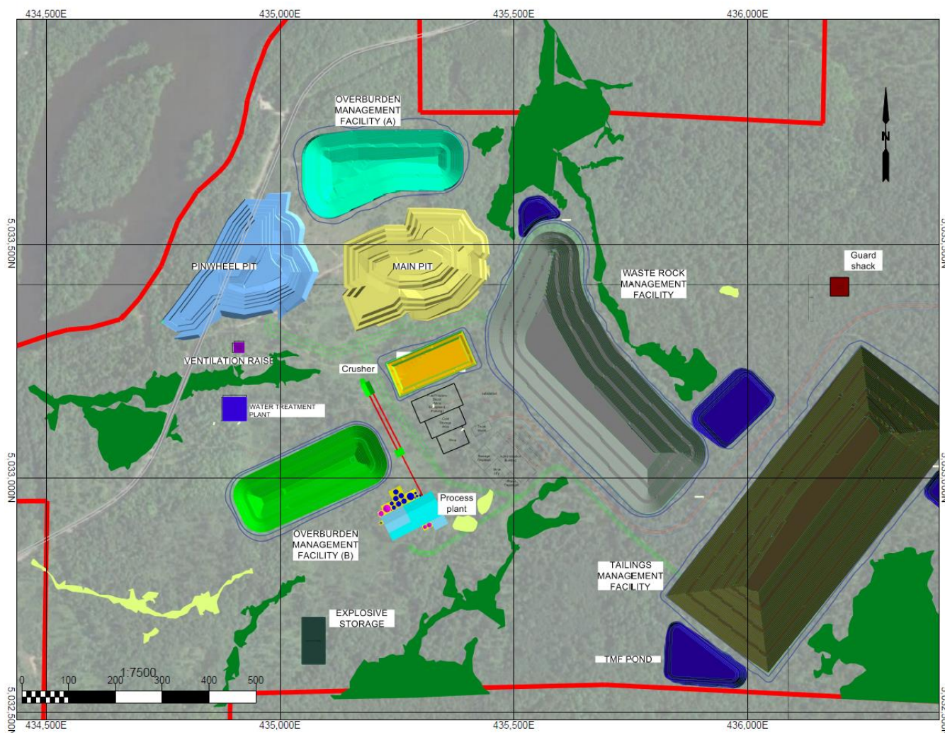
Figure 1-1: Back Forty Project Layout
