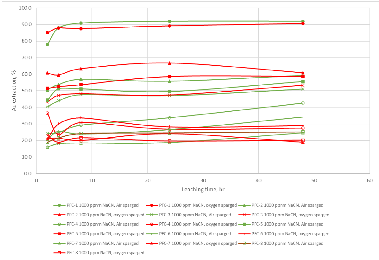
Figure 13-24: Leaching Performance Under Air and Oxygen Sparge
