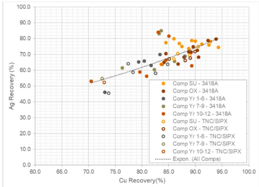
Figure 13-7: Copper Rougher Stage – Au Recovery Versus Cu Recovery
