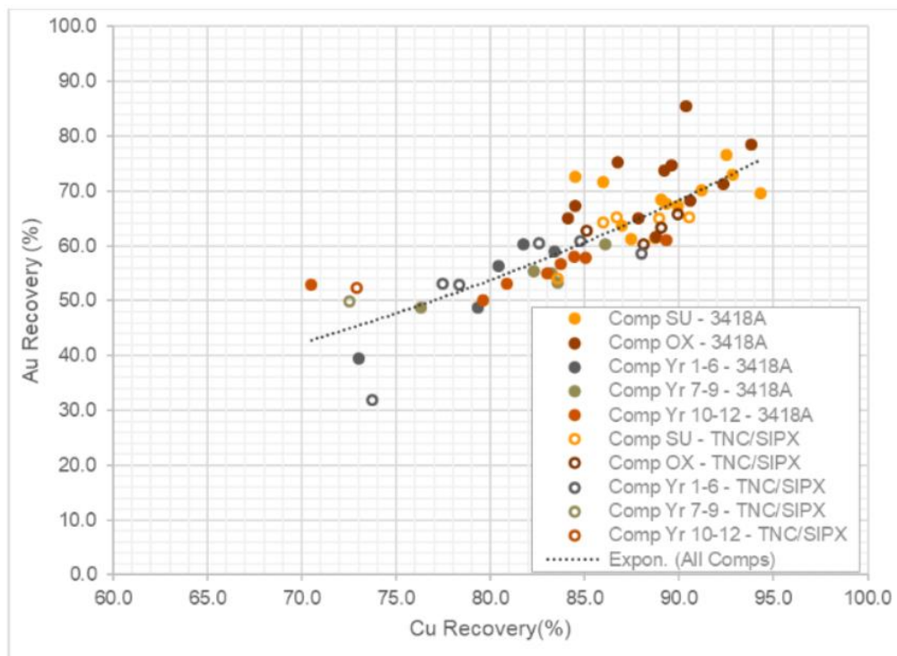
Figure 13-6: Copper Rougher Stage – Au Recovery Versus Cu Recovery
