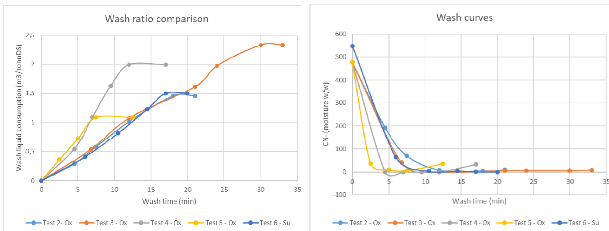
Figure 13-14: Wash Ratio Comparison and Wash Curves
