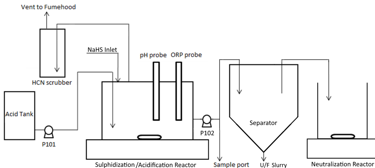
Figure 13-19: Schematic of Bench Scale SART Apparatus
