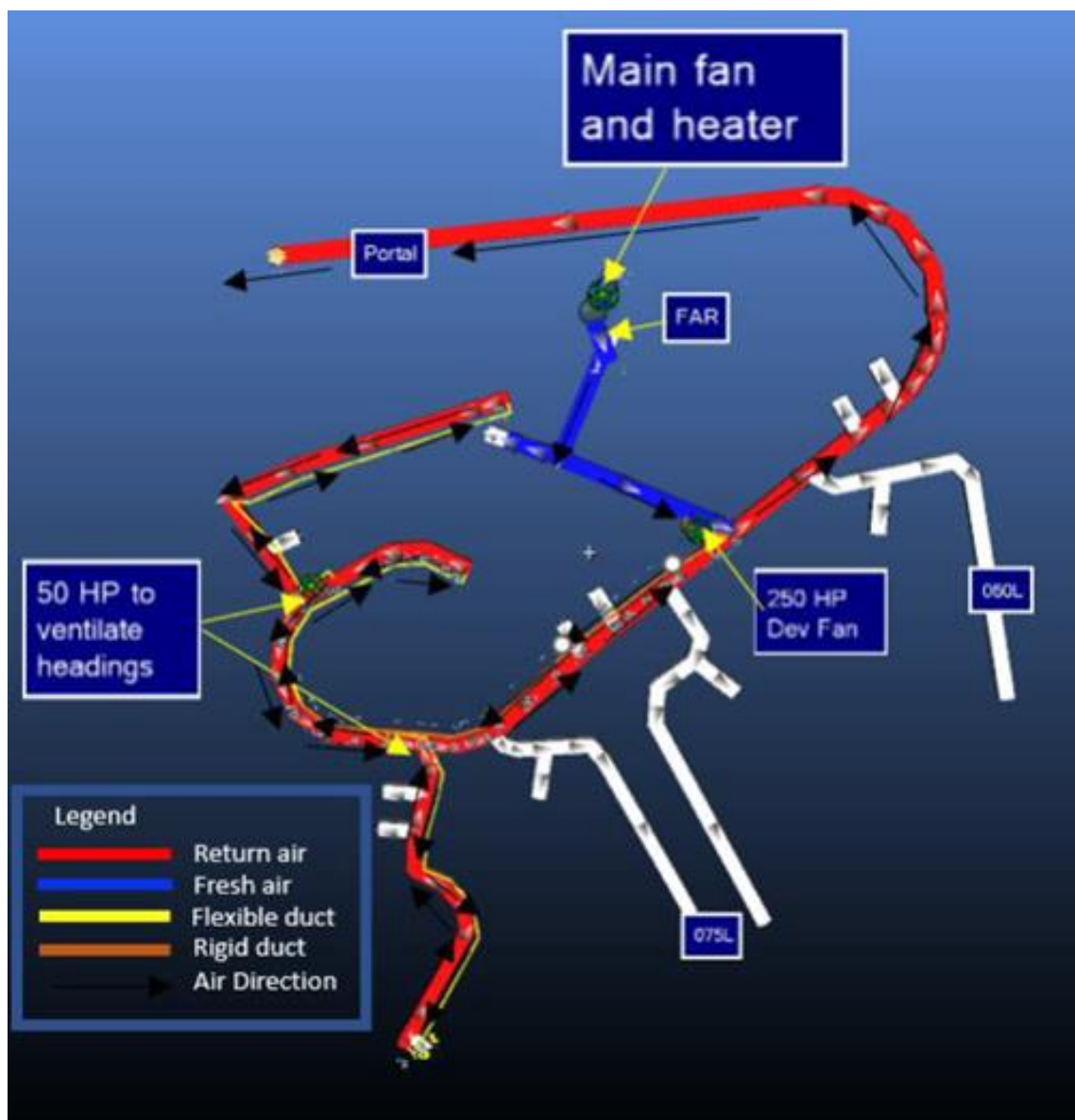
Figure 16-16: Plan View of Second Stage of Ventilation System
