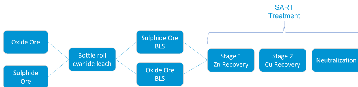
Figure 13-18: Block Diagram of the Overall Experimental Plan
