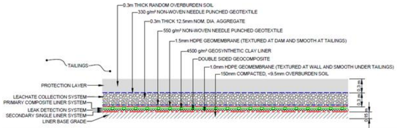
Figure 18-5: The Double Liner System of the TMF
