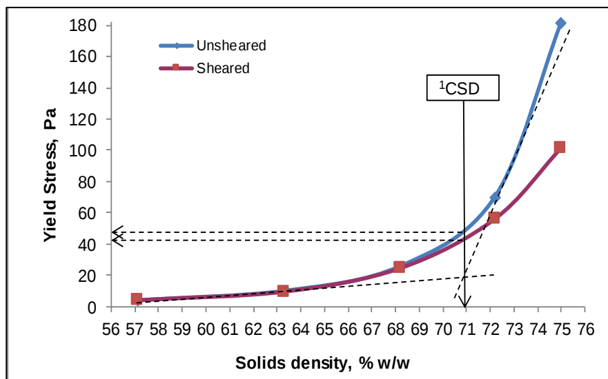
Figure 13-2: Solids Content Versus Yield Stress for PP-13 Bulk Clnr Conc Underflow
