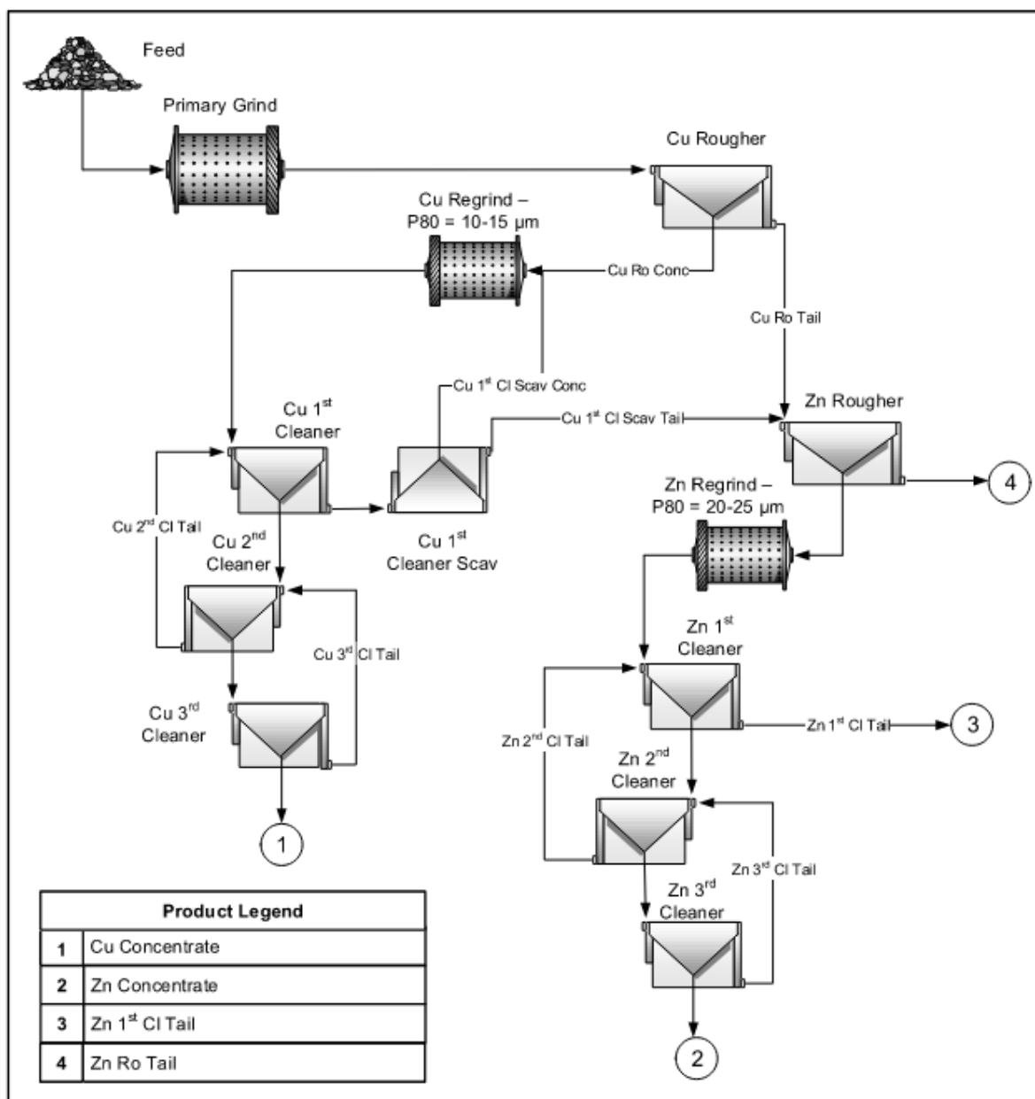
Figure 13-10: Locked Cycle Test Flowsheet
