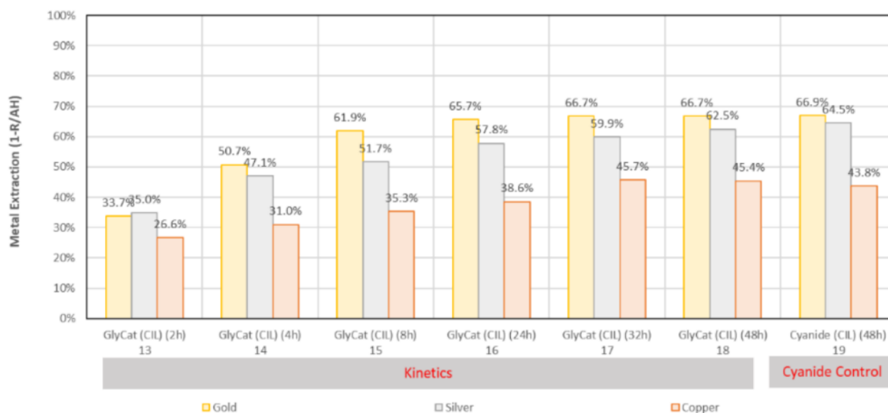
Figure 13-13: Metal Extraction Results – RLTs Round 3
