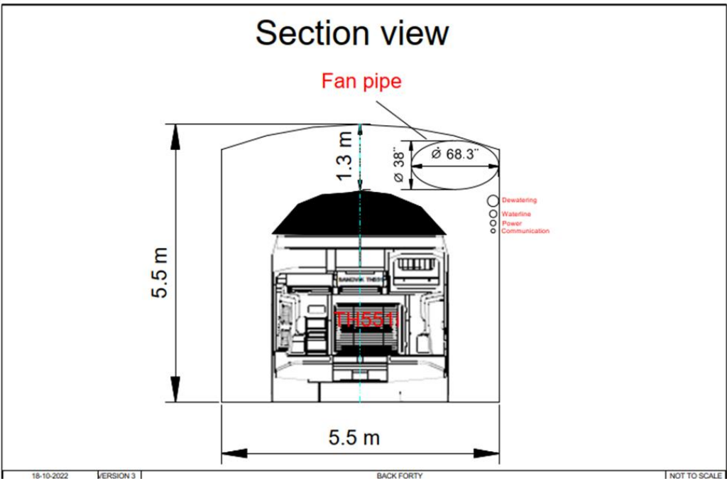
Figure 16-13: Typical Lateral Development Heading
