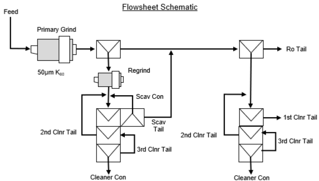
Figure 13-22: LCT Flowsheet
