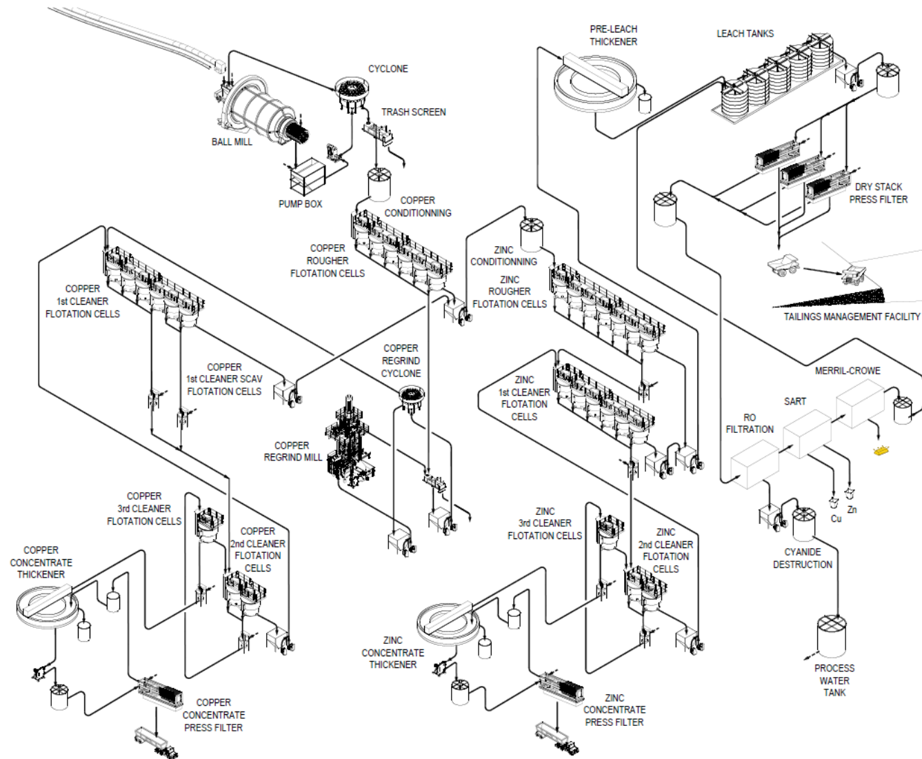
Figure 17-2: Process Flow Diagram (Processing section)
