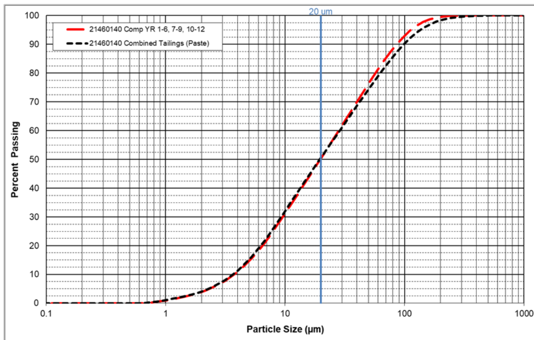
Figure 13-20: Particle Size Distribution
