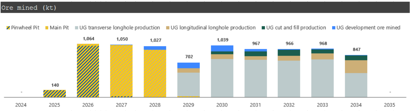
Figure 1-3: Back Forty Project Mining Schedule
