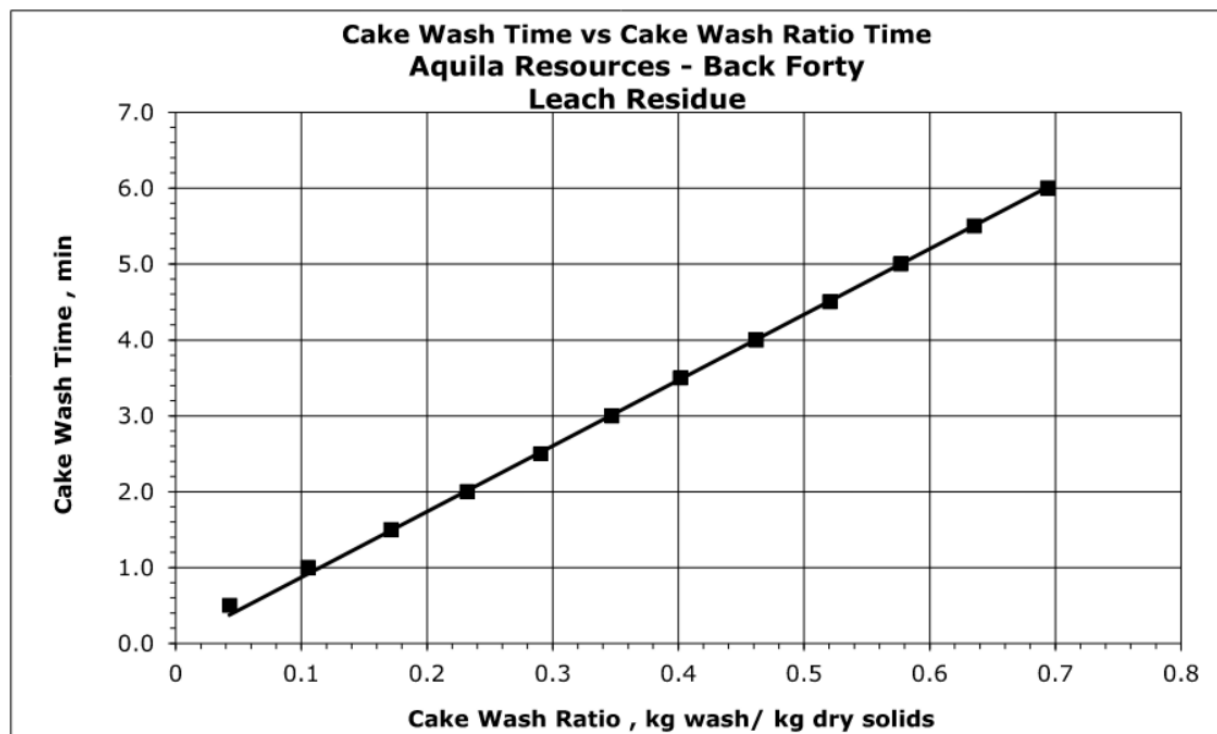
Figure 13-16: Cake Wash Time Versus Cake Wash Ratio Time – Aquila Resources – Back Forty – Leach Residue
