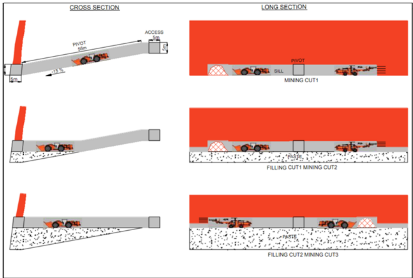
Figure 16-10: Cross-section of Typical Cut-and-Fill Stope
