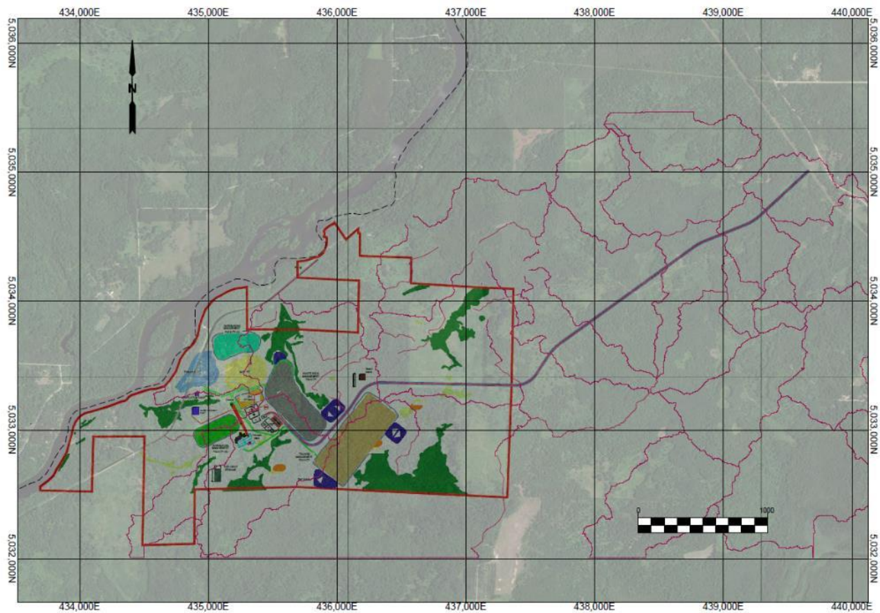
Figure 18-1: Infrastructure and Site Access Layout
