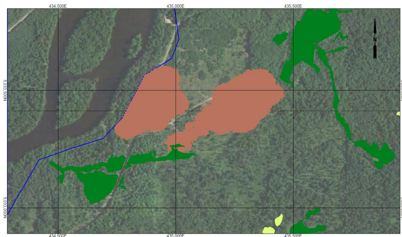
Figure 16-3: Revenue Factor 1 Pit Shell
