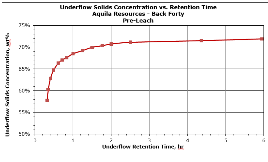
Figure 13-15: Underflow Solids Concentration Versus Retention Time – Aquila Resources – Back Forty
