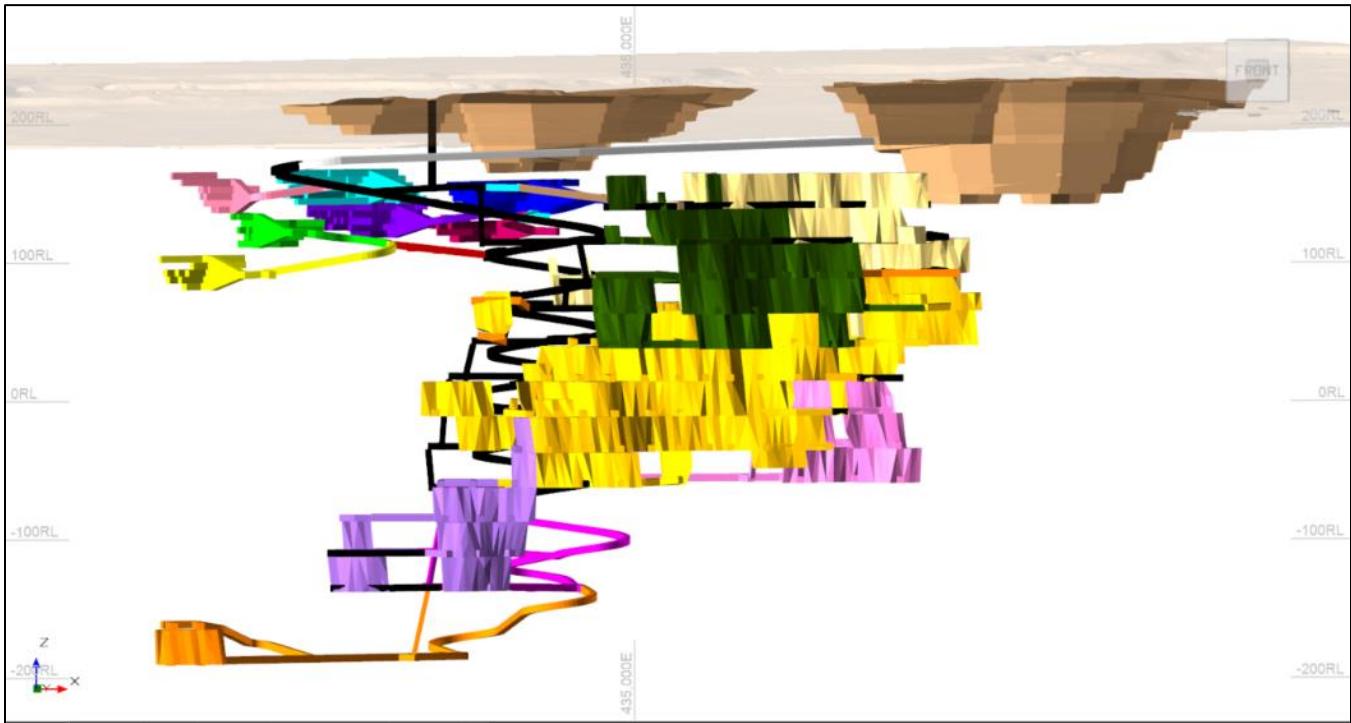
Figure 16-7: Open Pit and Underground Workings Looking North
