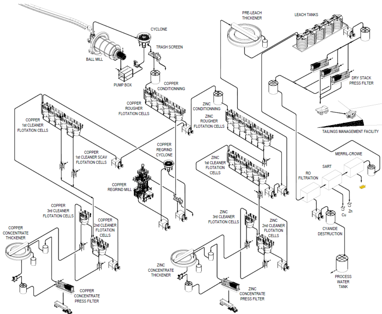
Figure 1-4: Process Flow Diagram (Processing section)
