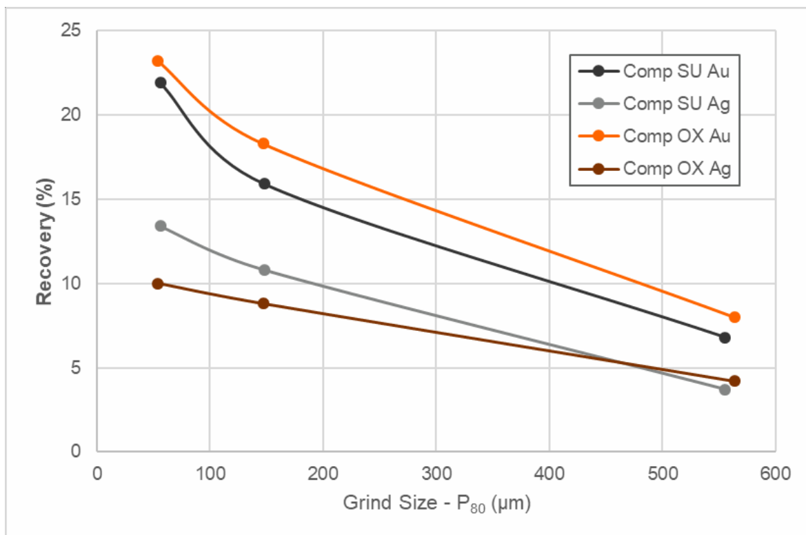
Figure 13-4: Au and Ag Recoveries Versus Grind Size
