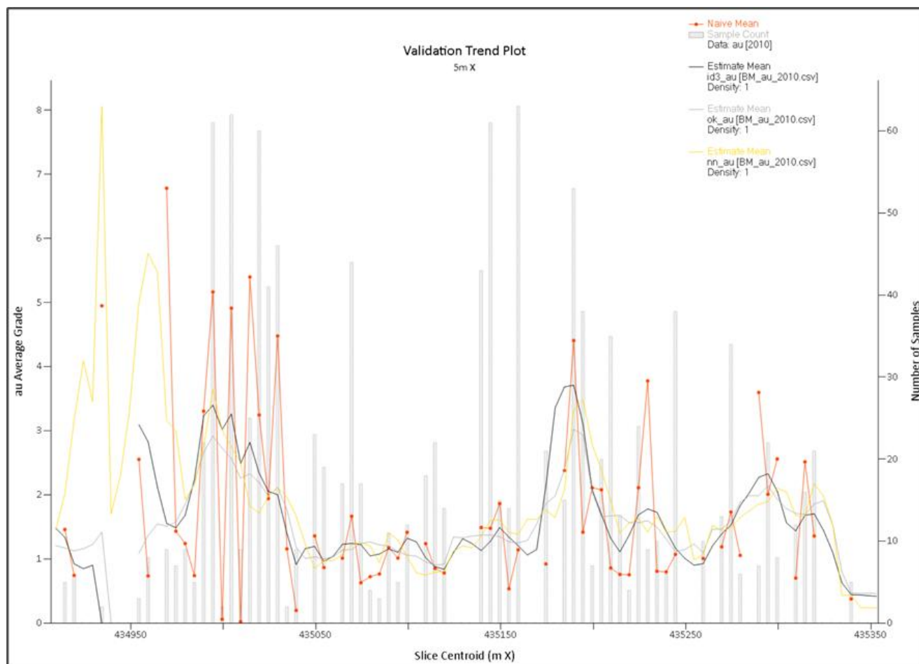
Figure 14-8: Validation Swath Plot of Zone 2010 for Gold (East Direction)
