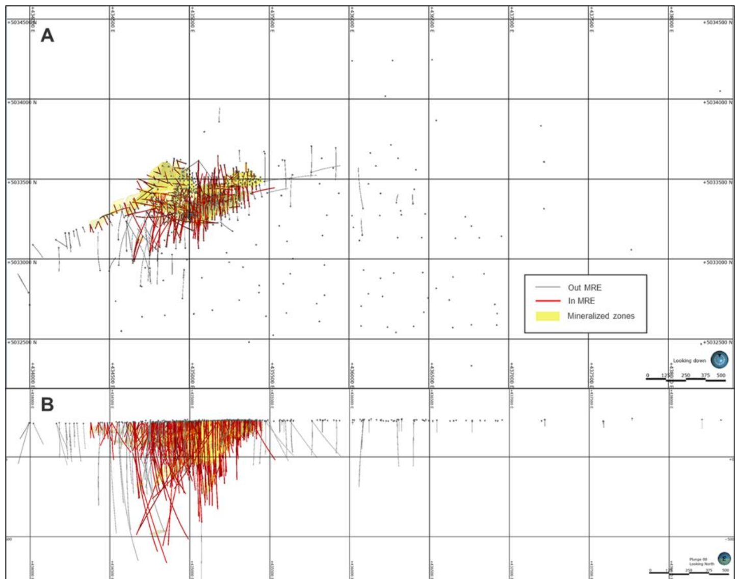
Figure 14-1: Surface Plan View (A) and Vertical Cross-Section Looking North (B) of the Validated DDH Used in the 2023 MRE
