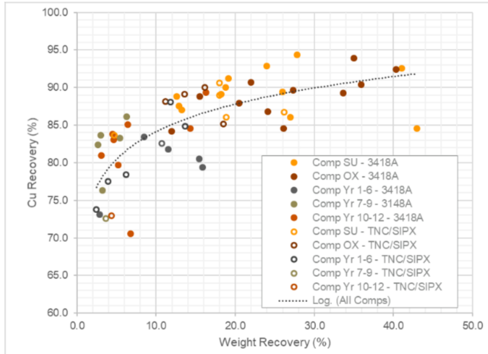
Figure 13-5: Copper Rougher Recovery Versus Weight Recovery – All Composites
