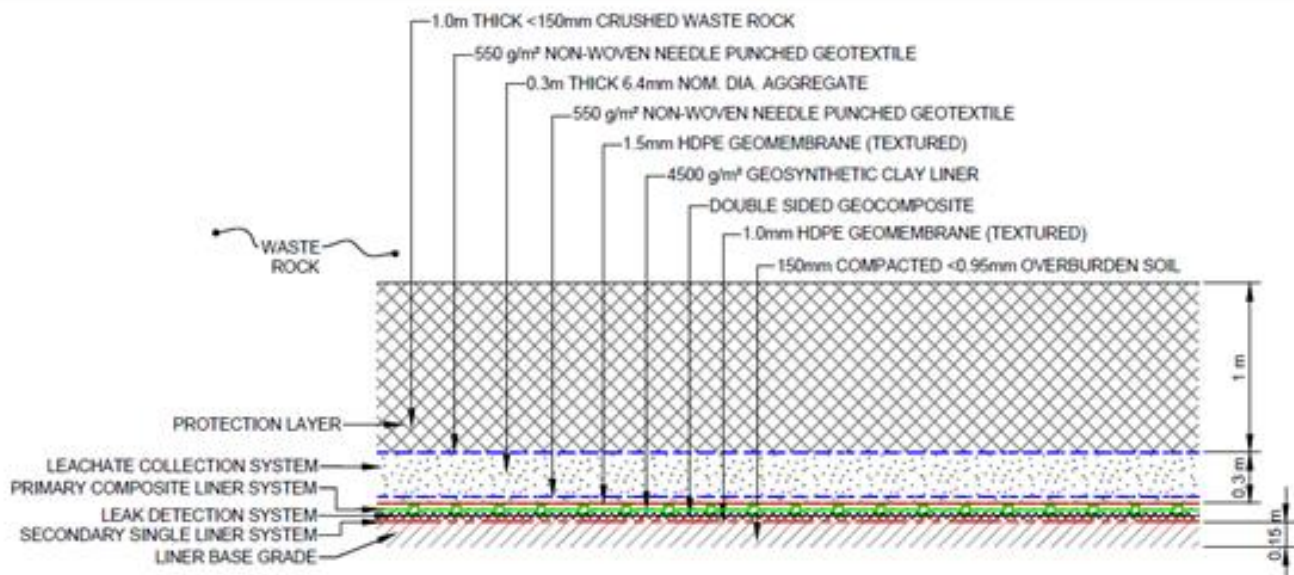
Figure 18-8: The Double Liner System of the WRMF
