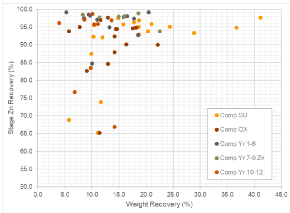
Figure 13-9: Zinc Rougher Stage Performance
