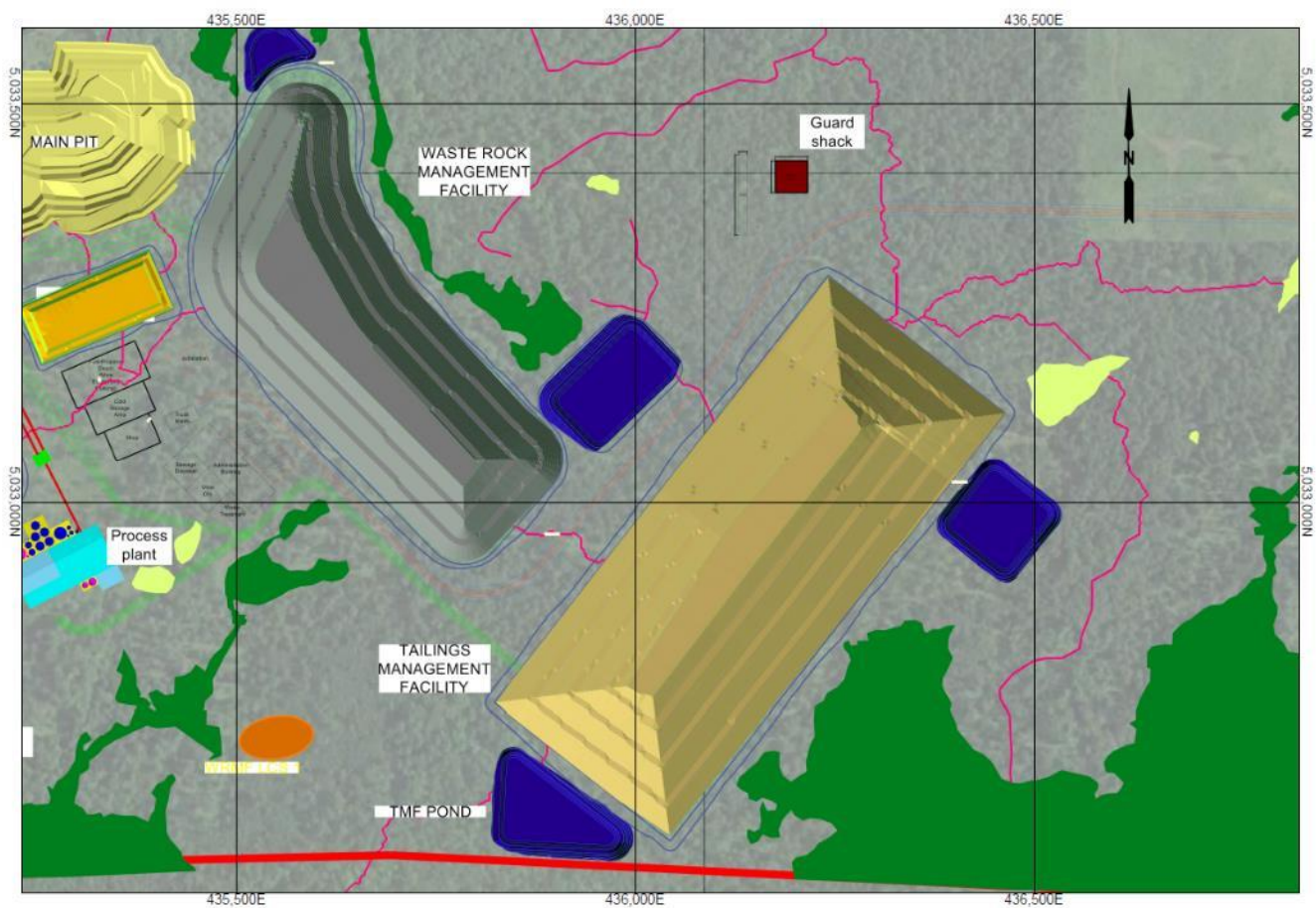
Figure 18-3: Plan View of the TMF
