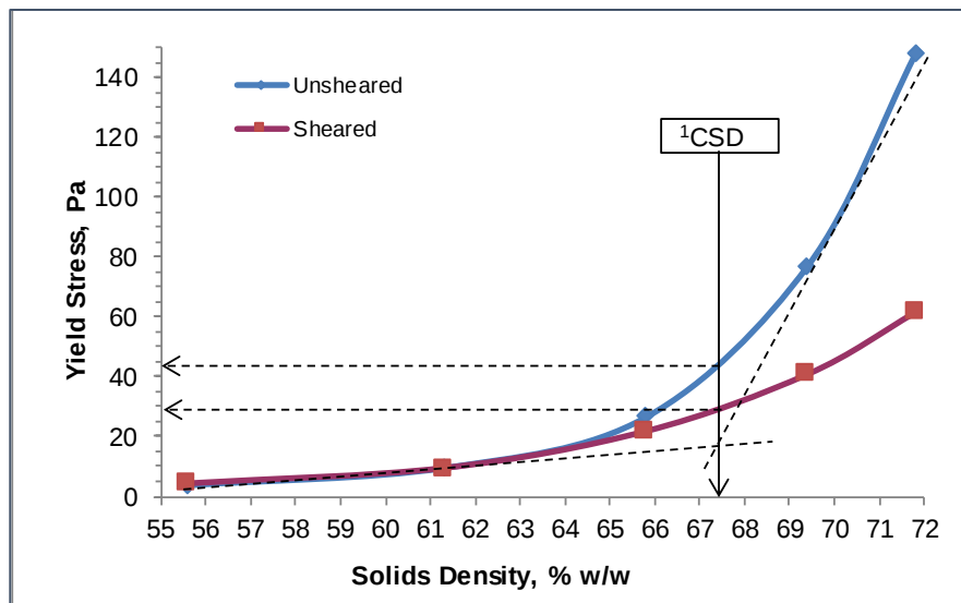
Figure 13-1: Solids Content Versus Yield Stress for PP-07 Zn Clnr Conc Underflow
