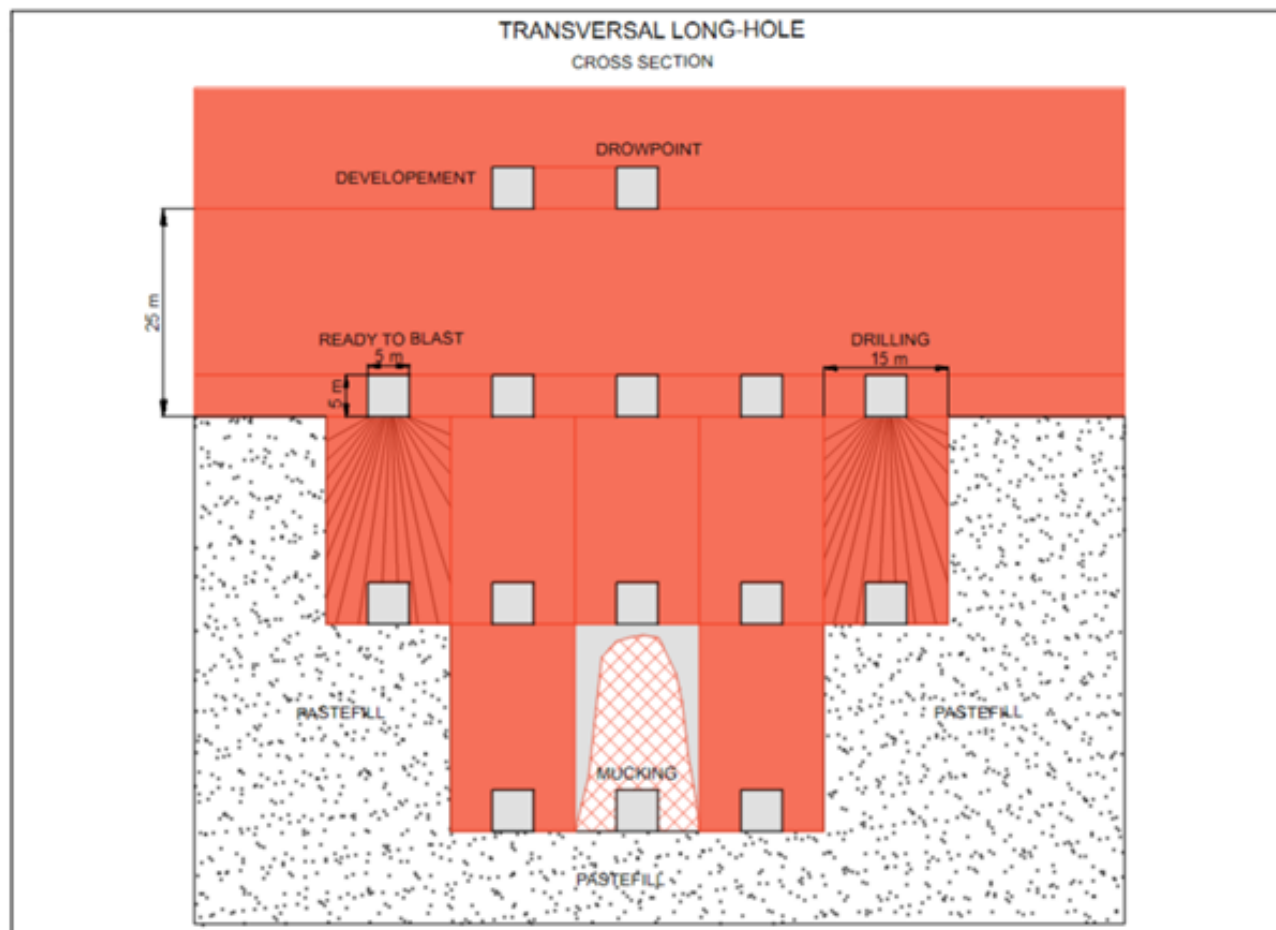
Figure 16-12: Sectional View of a Typical Transverse Longhole Stope
