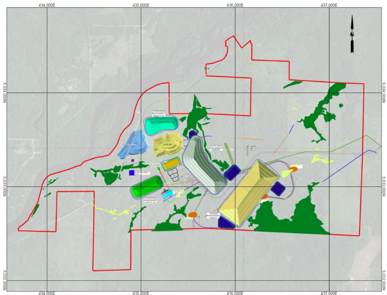
Figure 18-2: Site Infrastructure Layout
