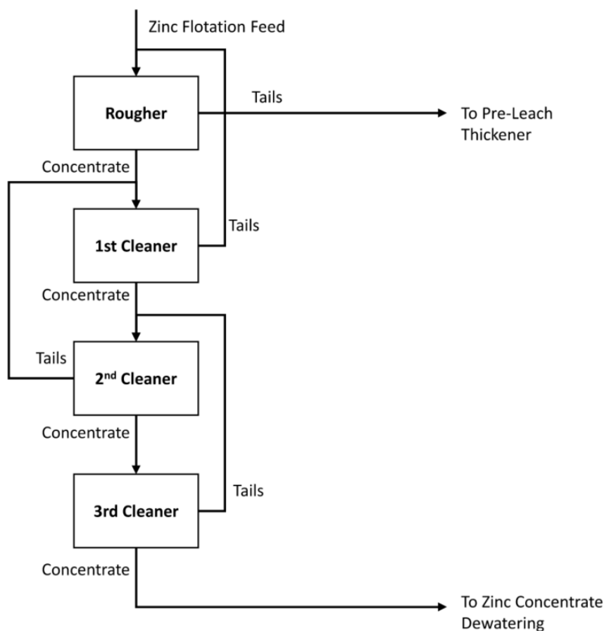
Figure 17-4: Zinc Flotation Circuit
