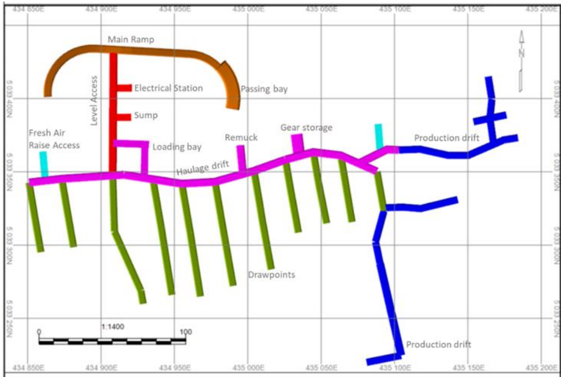
Figure 16-14: Typical Level Development
