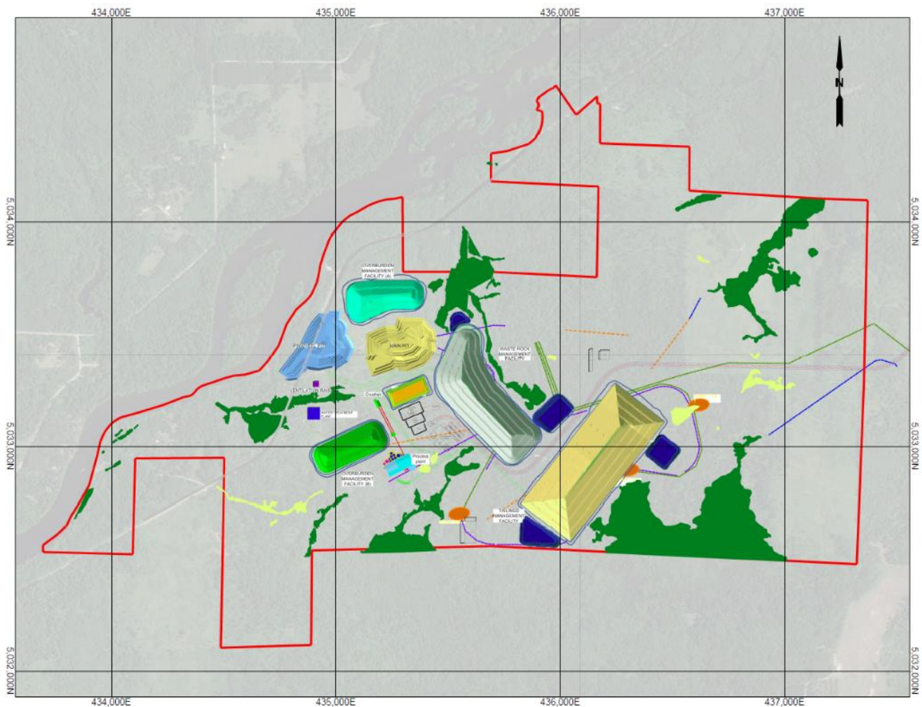
Figure 20-2: Back Forty Project Infrastructures
