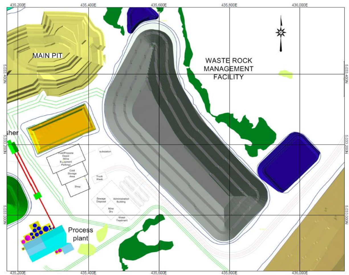
Figure 18-6: Plan View of WRMF
