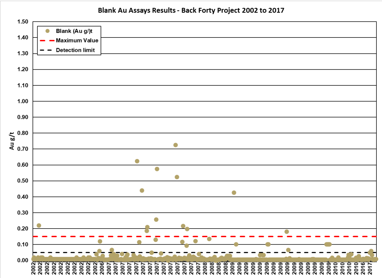
Figure 11-1: 2002-2017 Gold Results for Blanks (n=562) Assayed for the Project
