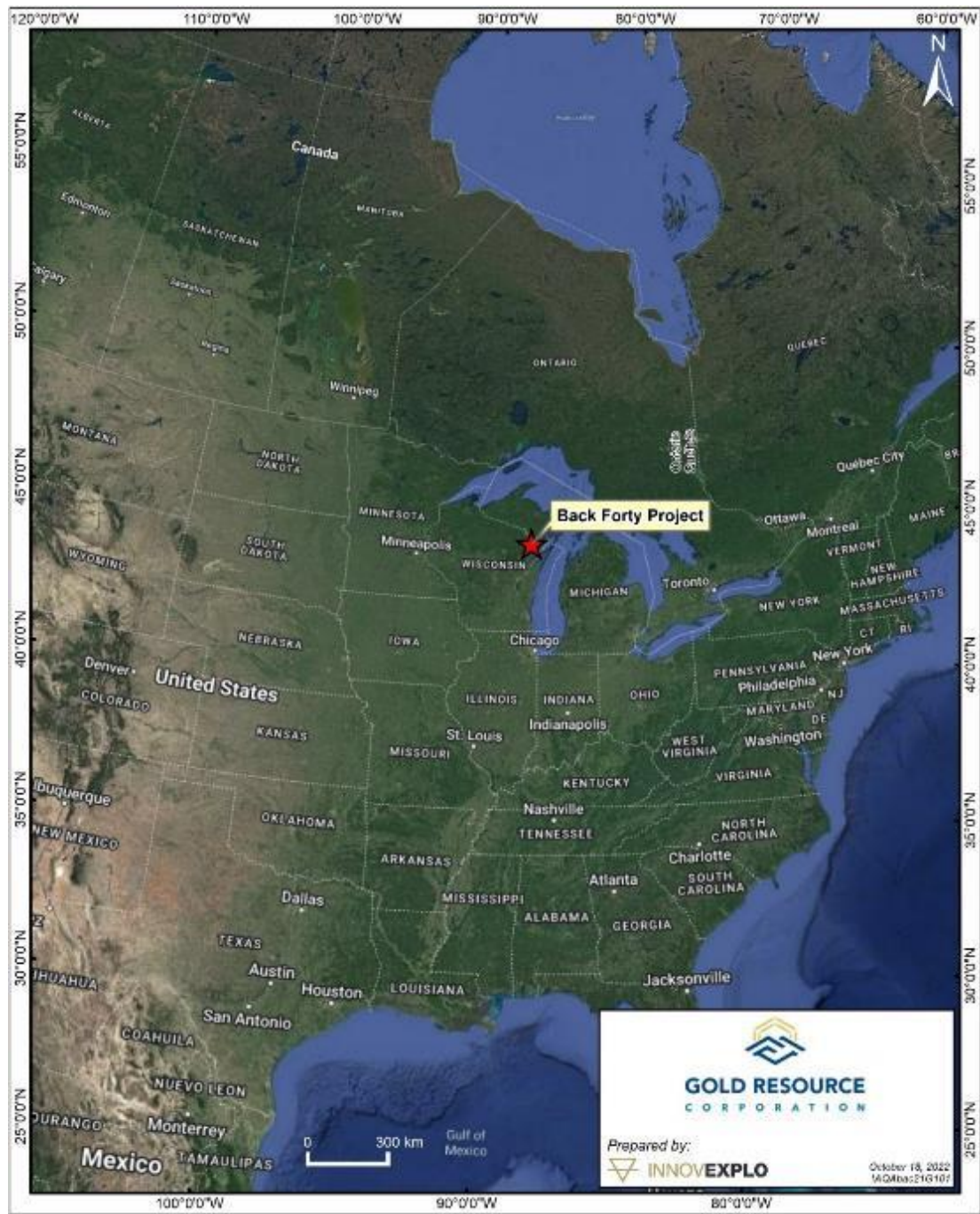
Figure 4-1: Location of the Back Forty Project
