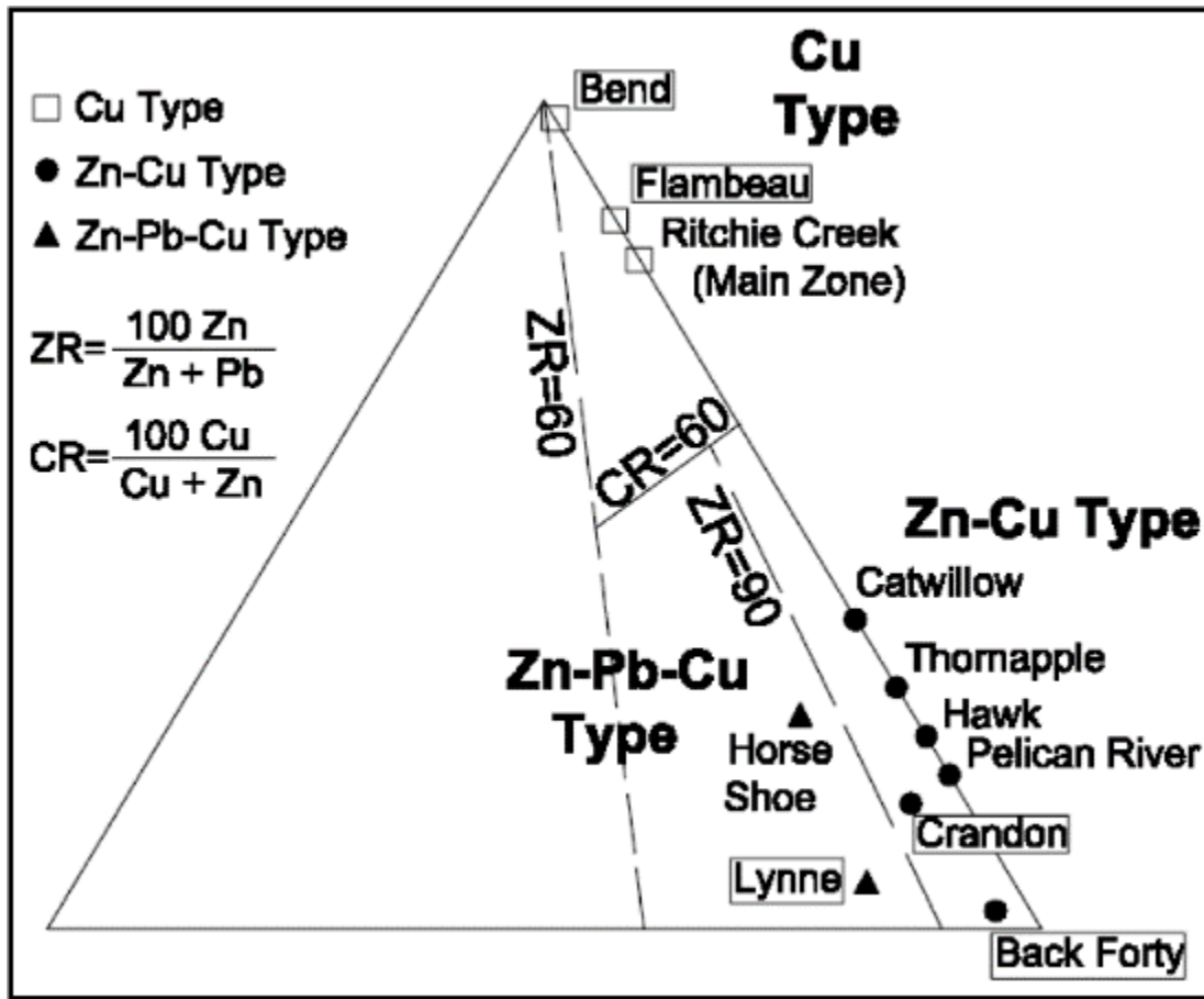
Figure 7-4: Classification of VMS Deposits in the PVB Based on Cu and Zn Ratios
