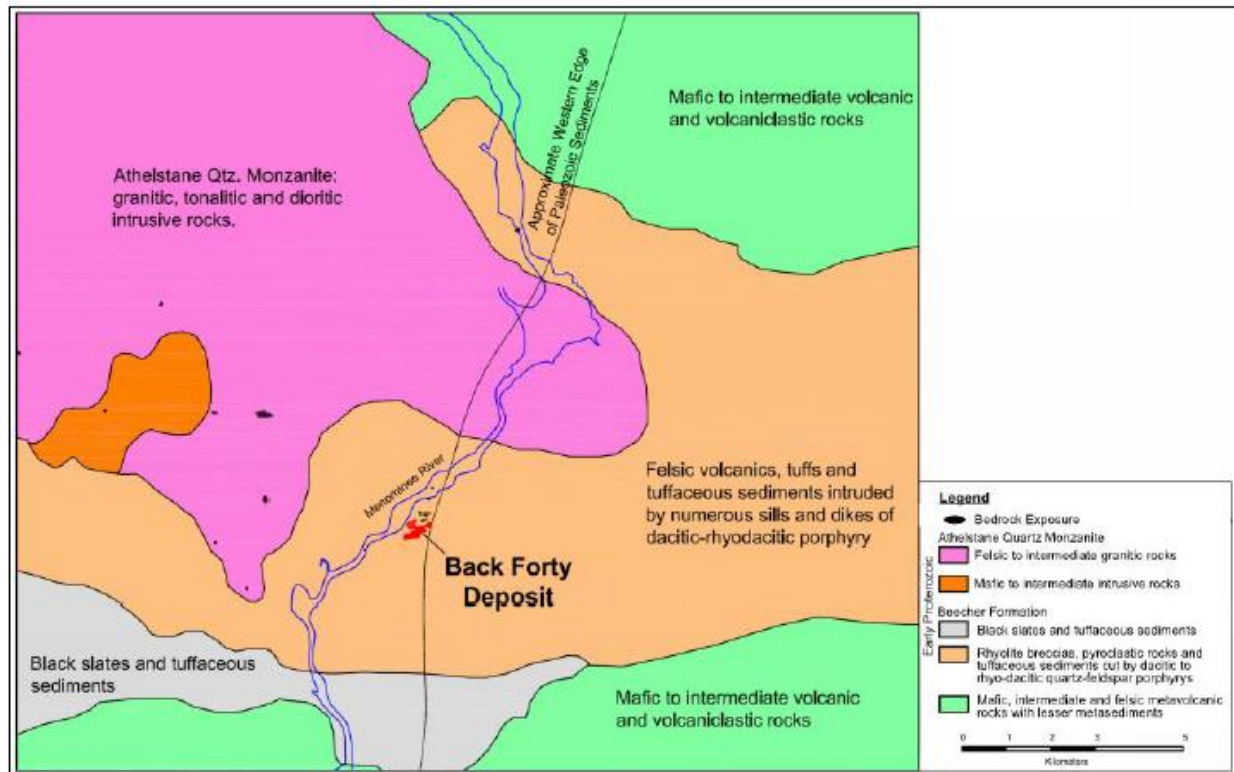
Figure 7-5: Geologic Map of the Back Forty Area
