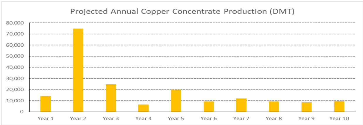
Figure 19-3: Projected Annual Copper Concentrate Production
