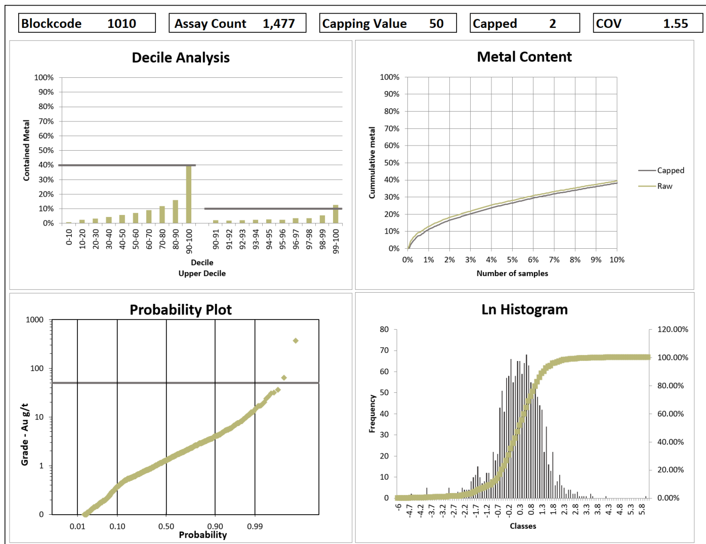
Figure 14-4: Example of Graphs Supporting a Capping Value of 50 G/T Au for the 1010 Zone
